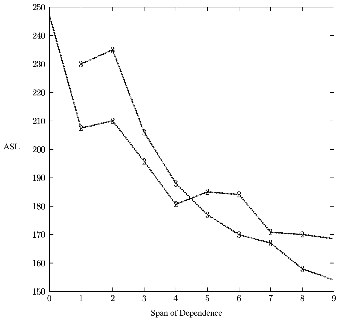
Figure 2: Average Search Length where the dependence is limited to pairwise dependence (represented by “2”) or to term triples (“3”) when estimating \Pr(d|rel) . Independence is assumed for \Pr(d) .
