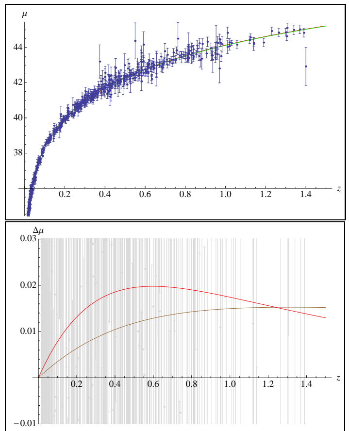
FIG. 1: Top panel: Hubble plot of distance modulus \mu versus redshift z for the \Lambda CDM ( w = -1 ) model (green) and models 1 (brown) and 2 (red). The lines are essentially indistinguishable. Bottom panel: The \Lambda CDM model is subtracted from models 1 (brown) and 2 (red). The \Lambda CDM model is, by definition, represented by the \Delta\mu = 0 axis. As can be judged by the size of the error bars of the data, all are excellent fits to the supernovae data. (The color plots are in the online version of the paper.)
