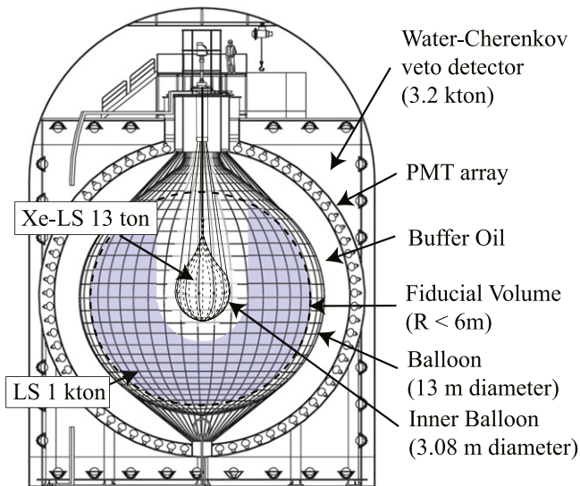
Figure 1. Schematic diagram of the KamLAND detector. The shaded region in the liquid scintillator indicates the volume for the \bar{\nu}_e analysis after the IB installation.
