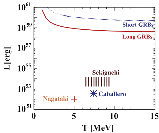
Figure 5. KamLAND constraint on the luminosity ( L ) and effective temperature ( T ) relation in the GRB accretion disk, together with several theoretical calculations (Nagataki & Kohri 2002; Caballero et al. 2009; Sekiguchi & Shibata 2011).
