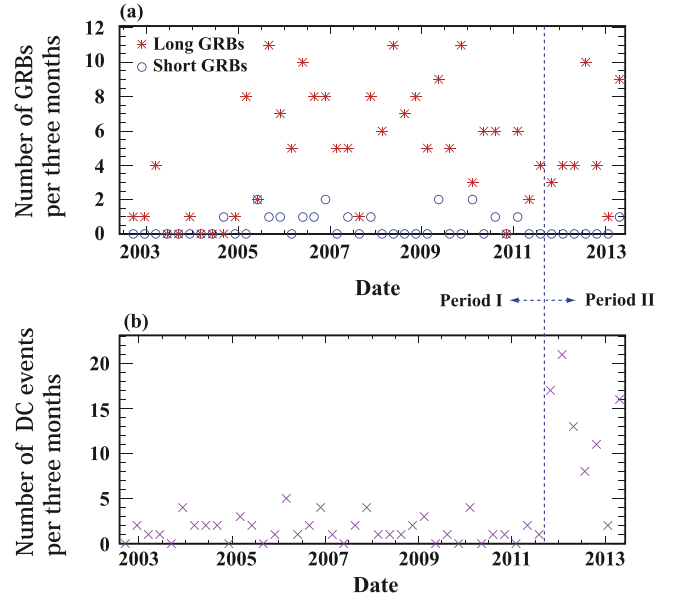
Figure 2. Number of long and short GRBs per 3 months (upper panel) and DC events per 3 months (bottom panel). The number of GRBs significantly increased due to the SWIFT satellite after 2004 December. During Period I, the DC event rate is within the statistical uncertainty. Period II started in 2011 September and allowed for a lower energy threshold, increasing the number of DC events.
