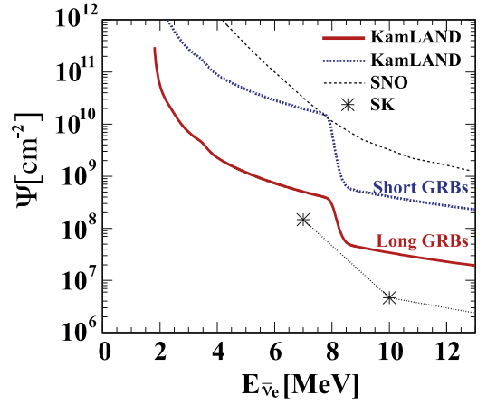
Figure 4. Fluence upper limits on \bar{\nu}_e from GRBs as a function of neutrino energy. Results from SK and SNO are also presented for comparison. SK is expected to have poorer sensitivity at low energies due to the detection threshold. Below 7 MeV, KamLAND establishes the tightest limits on neutrino fluence. The slight distortion around 3–4 MeV is from the energy dependence of the selection efficiency ( \epsilon_s^{\text{II}} ).
