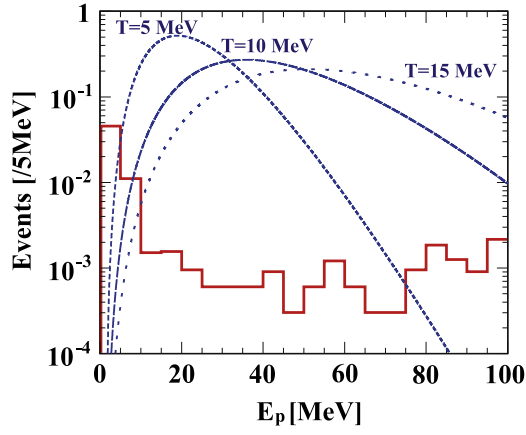
Figure 3. Combined background spectrum of Periods I and II (solid red). The integral is 7.4 \times 10^{-2} events. The dashed curves provide our 90% upper limits under the assumption of a Fermi–Dirac distribution at temperature T of \bar{\nu}_e . Each dashed curve from the left to the right corresponds to T = 5, 10, 15 MeV.
