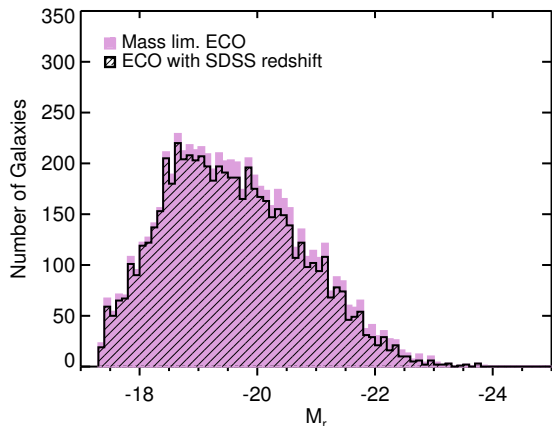
FIG. 4.— Illustration of the additional completeness of the final M_{bary} -limited ECO catalog over the SDSS redshift catalog. The M_r distribution of the ECO sample in our reprocessed magnitude system (see §3.1 for details) is indicated by the purple solid histogram, and the distribution of ECO galaxies that have SDSS redshifts is indicated by the black hashed histogram.
