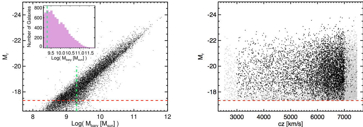
FIG. 3.— Illustration of the selection of the ECO catalog. Panel a shows the M_r and M_{bary} distributions of the initial ECO catalog (dots and purple inset M_{bary} histogram), where the horizontal red line indicates the M_r < -17.33 redshift completeness limit and the vertical green lines indicate the final mass cut we adopt to create an approximately baryonic mass limited sample to M_{bary} > 10^{9.3} M_\odot . Panel b shows the magnitude and cz limits of ECO, where light grey dots indicate the M_r < -17.33 sample and black dots indicate our final approximately mass-limited sample with M_{bary} > 10^{9.3} M_\odot and group membership within the ECO volume.
