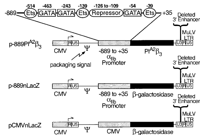
Fig. 1. Schematic diagram of the retroviral plasmid constructs. Transgene cassettes were inserted between the LTR-containing elements (U3, R, U5) of a MuLV-derived vector. The MuLV enhancer region was deleted from a sequence (U3) of the 3' LTR (15), and the \alpha IIB promoter (nucleotides -889 to +35) was used to direct expression of the PI A2 \beta 3 or \beta -gal (nLacZ) in transduced cells. This \alpha IIB promoter segment contains sequences necessary for megakaryocyte-specific expression (7). The immediate-early enhancer/promoter region of the CMV drives gene transcription for retroviral production in the 293 cells (see Materials and Methods ). As a positive control, the CMV promoter was used to drive nonspecific expression of \beta -gal in cells transduced with virions produced from vector pCMVnLacZ.
