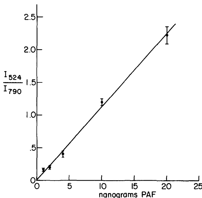
Fig. 4. Plot of the ratio of ion intensities at 524 m/z ( I_{524} ) and 790 m/z ( I_{790} ) for samples containing 1- O -hexadecyl-2- O -acetyl- sn -glycero-3-phosphocholine and 1,2-dioctadecanoyl- sn -glycero-3-phosphocholine. See Materials and Methods for details.
