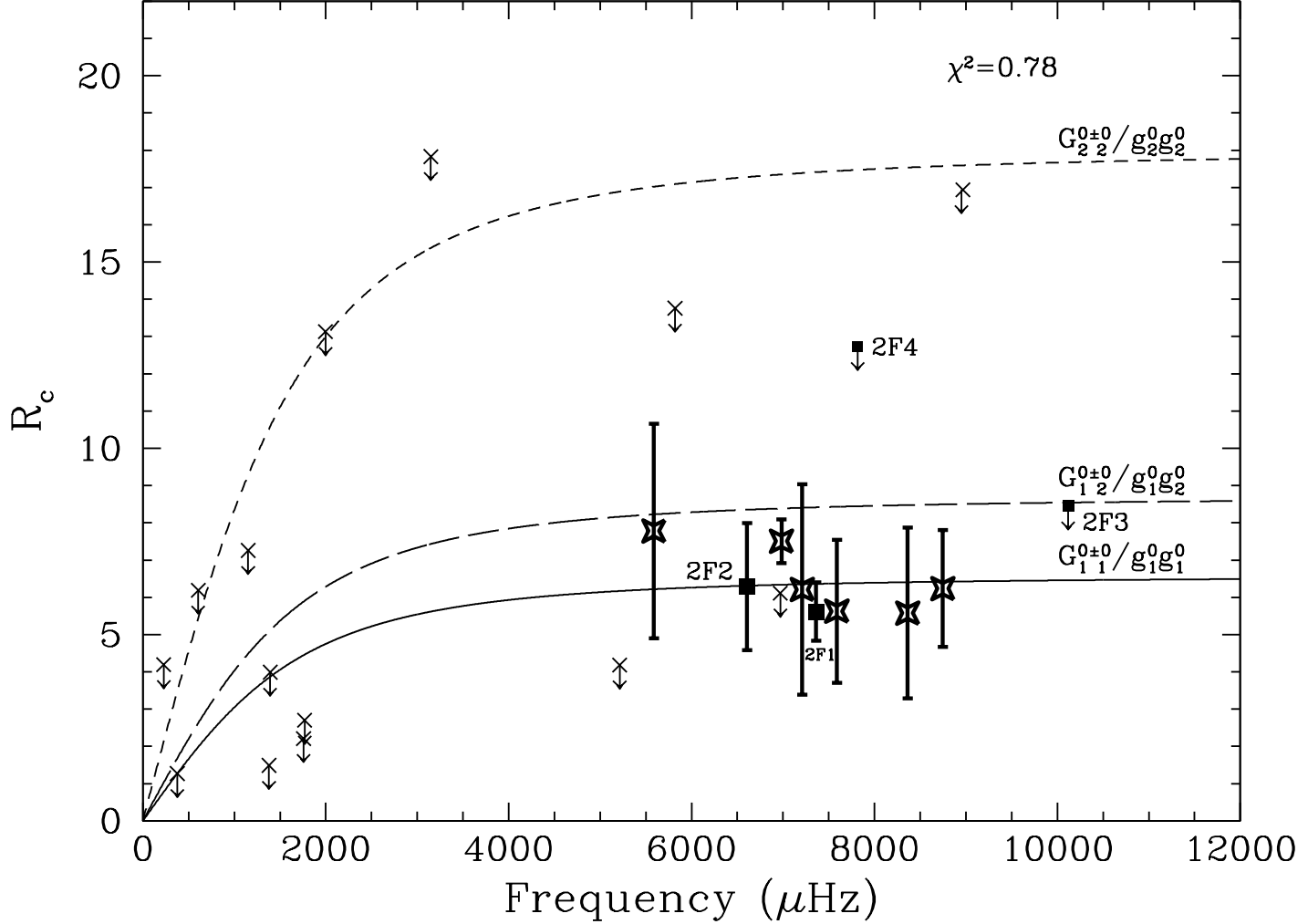
Fig. 8.— Ratio of combination to parent mode amplitudes ( R_c ) for GD 66. The lines are theoretical predictions for G_{11}^{0+0}/g_{11}^0g_1^0(\Theta_o = 13^\circ) (solid line), G_{12}^{0+0}/g_{11}^0g_2^0(\Theta_o = 13^\circ) (long-dashed line), and G_{22}^{0+0}/g_2^0g_2^0(\Theta_o = 13^\circ) (dashed line). The data points are the detected harmonics or limits (filled squares), detected cross combination frequencies (stars), and limits for the cross combinations (crosses). The downward arrows on the limits indicate that the points represent maximum values. The upper limit for R_c of 2F5 lies at 124 (not shown).
