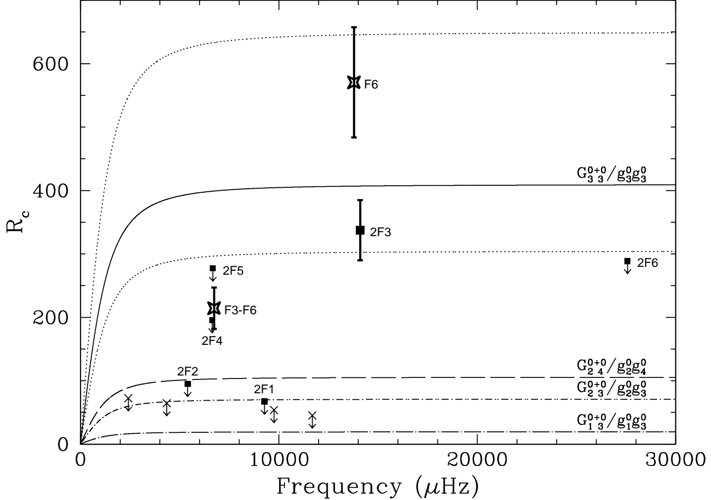
Fig. 15.— Ratio of combination to parent mode amplitudes ( R_c ) for G185-32. The lines are theoretical predictions for G_3^{0+0}/g_3^0g_3^0(\Theta_o = 13^\circ) (solid line), G_2^{0+0}/g_2^0g_4^0(\Theta_o = 13^\circ) (long-dashed line), G_2^{0+0}/g_2^0g_3^0(\Theta_o = 13^\circ) (dot-dashed line), and G_1^{0+0}/g_1^0g_3^0(\Theta_o = 13^\circ) (dot-long-dashed line). The data points are the detected harmonics or limits (filled squares), detected cross combination frequencies (stars), and limits for the cross combinations involving the F3 pulsation mode only (crosses). The downward arrows on the limits indicate that the points represent maximum values. The dotted lines on either side of the \ell_i = \ell_j = 3 line are the R_c predictions for extremum in inclination: \Theta_o = 20^\circ (top) and \Theta_o = 0^\circ (bottom). Wu’s predictions for G_4^{0+0}/g_4^0g_4^0(\Theta_o = 13^\circ) are not shown because they reach values above R_c \sim 3600 .
