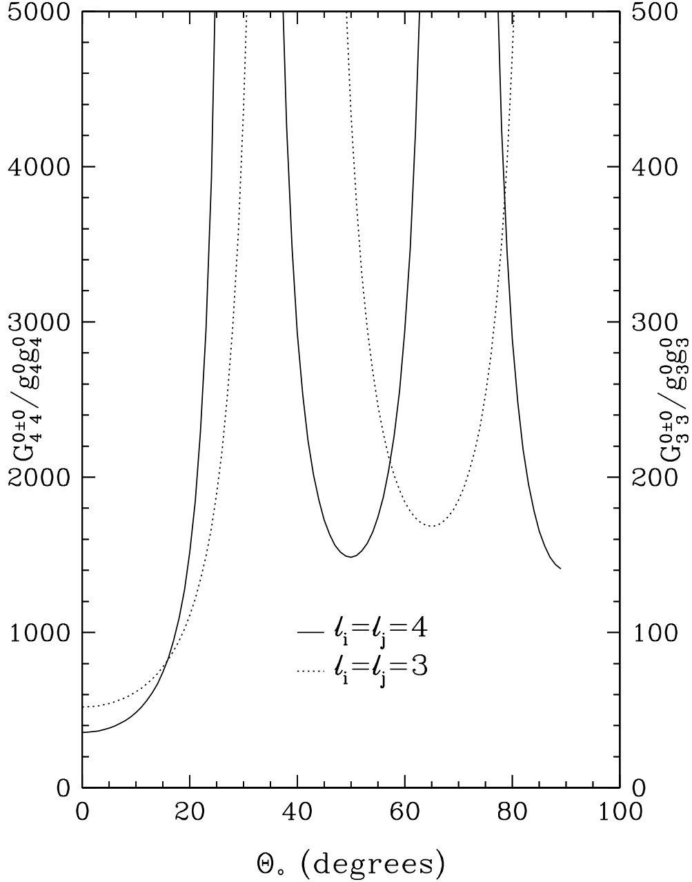
Fig. 22.— \mathcal{G} with m_i = m_j = 0 (see equation 9) plotted as a function of inclination angle ( \Theta_0 ). The scale of \mathcal{G} for l_i = l_j = 4 (solid line) is a factor of ten larger than the scale of \mathcal{G} for l_i = l_j = 3 (dotted line). The predicted amplitudes of the combination frequencies show a dramatic increase for inclinations greater than 20^\circ , and the predictions less than 20^\circ increase more rapidly than the cases for \ell = 1 and 2 (see Figures 2 and 3).
