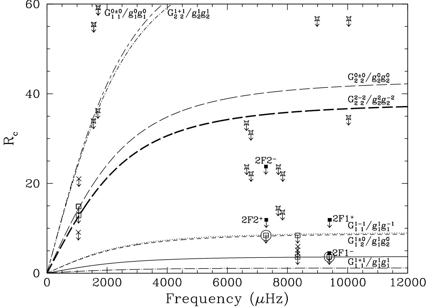
Fig. 20.— Ratio of combination to parent mode amplitudes ( R_c ) for R548. The lines are theoretical predictions for G_{1\ 1}^{0\pm 0}/g_1^0 g_1^0 ( \Theta_o = 79^\circ ) (long-short-dashed line), G_{2\ 2}^{1+1}/g_2^1 g_2^1 ( \Theta_o = 79^\circ ) (dot-dashed line), G_{2\ 2}^{0\pm 0}/g_2^0 g_2^0 ( \Theta_o = 79^\circ ) (long-dashed line), G_{2\ 2}^{2-2}/g_2^2 g_2^{-2} ( \Theta_o = 79^\circ ) (bold long-dashed line), G_{1\ 1}^{1-1}/g_1^1 g_1^{-1} ( \Theta_o = 79^\circ ) (dotted line), G_{1\ 2}^{1\pm 0}/g_1^1 g_2^0 ( \Theta_o = 79^\circ ) (dashed line), G_{1\ 1}^{1+1}/g_1^1 g_1^1 ( \Theta_o = 79^\circ ) (solid line), G_{1\ 1}^{1\pm 0}/g_1^1 g_1^0 ( \Theta_o = 79^\circ ) (solid line, not labeled because of space), and G_{2\ 2}^{2+2}/g_2^2 g_2^2 ( \Theta_o = 79^\circ ) (dot-long-dashed line, not labeled). The data points are the limits on the harmonics (filled squares), limits for the same- m cross combinations (crosses), limits for the different- m cross combinations (open squares), and limits for the cross combinations between one of the doublet modes (F1 or F2) and one of the lower amplitude singlet modes (stars). The downward arrows on the limits indicate that the points represent maximum values. The open square limits for F1^-+F1^+ and F2^-+F2^+ are circled for easier identification.
