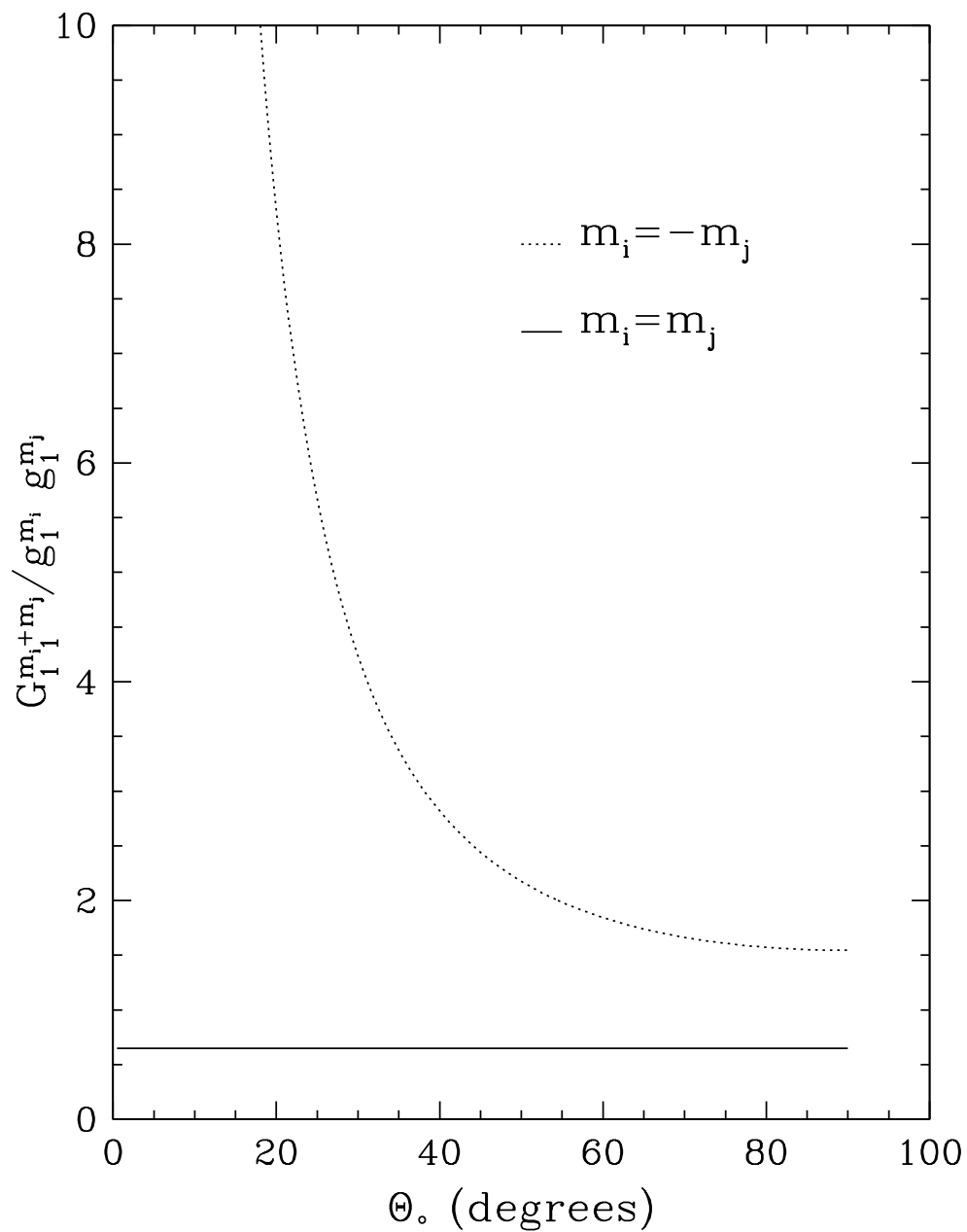
Fig. 3.— \mathcal{G} with l_i = l_j = 1 and m_i + m_j (see equation 9) plotted as a function of inclination angle ( \Theta_0 ). The amplitude of the combination frequencies is insensitive to inclination when \Theta_0 \gtrsim 60^\circ for m_i = -m_j (dotted line). When both parent modes have the same m (solid line), the combination amplitude is always independent of inclination. \mathcal{G} with m_i - m_j can be obtained by letting the dotted line represent m_i = m_j and the solid line represent m_i = -m_j .
