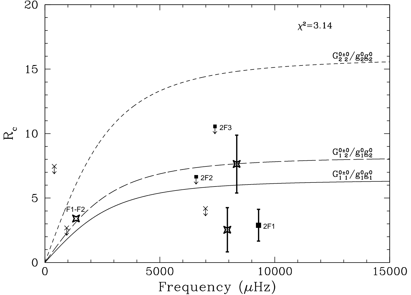
Fig. 14.— Ratio of combination to parent mode amplitudes ( R_c ) for G117-B15A. The lines are theoretical predictions for G_{11}^{0+0}/g_1^0g_1^0(\Theta_o = 5^\circ) (solid line), G_{12}^{0+0}/g_1^0g_2^0(\Theta_o = 5^\circ) (long-dashed line), and G_{22}^{0+0}/g_2^0g_2^0(\Theta_o = 5^\circ) (dashed line). The data points are the detected harmonics or limits (filled squares), detected cross combination frequencies (stars), and limits for the cross combinations (crosses). The downward arrows on the limits indicate that the points represent maximum values. There are no error bars for F1-F2 because there were none reported by Kepler et al. (1995b).
