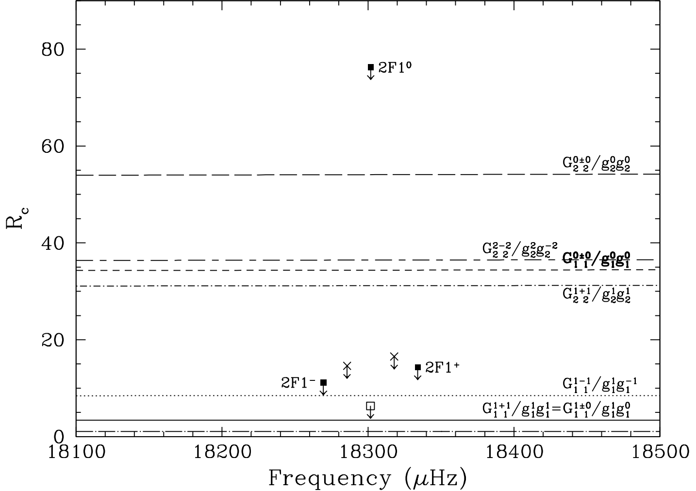
Fig. 21.— Ratio of combination to parent mode amplitudes ( R_c ) for G226-29. The lines are theoretical predictions for G_{2,2}^{0±0}/g_{2,2}^0g_2^0(\Theta_o = 74^\circ) (long-dashed line), G_{2,2}^{2-2}/g_{2,2}^2g_2^{-2}(\Theta_o = 74^\circ) (long-short-dashed line), G_{1,1}^{0±0}/g_1^0g_1^0(\Theta_o = 74^\circ) (dashed line), G_{2,2}^{1+1}/g_2^1g_2^1(\Theta_o = 74^\circ) (dot-dashed line), G_{1,1}^{1-1}/g_1^1g_1^{-1}(\Theta_o = 74^\circ) (dotted line), G_{1,1}^{1+1}/g_1^1g_1^1(\Theta_o = 74^\circ) (solid line), G_{1,1}^{1±0}/g_1^1g_1^0(\Theta_o = 74^\circ) (solid line), and G_{2,2}^{2+2}/g_{2,2}^2g_2^2(\Theta_o = 74^\circ) (dot-long-dashed line, not labeled because of space). Theoretical lines for G_{2,2}^{2±0}/g_{2,2}^2g_2^0(\Theta_o = 74^\circ) and G_{2,2}^{1±0}/g_2^1g_2^0(\Theta_o = 74^\circ) are not shown because they are very near to the predictions for G_{1,1}^{1±0}/g_1^1g_1^0(\Theta_o = 74^\circ) . The data points are the limits on the harmonics (filled squares), a limit for the nonzero different- m cross combination (open square), and limits for the cross combinations between the m \neq 0 modes and the central m = 0 mode (crosses). The downward arrows on the limits indicate that the points represent maximum values.
