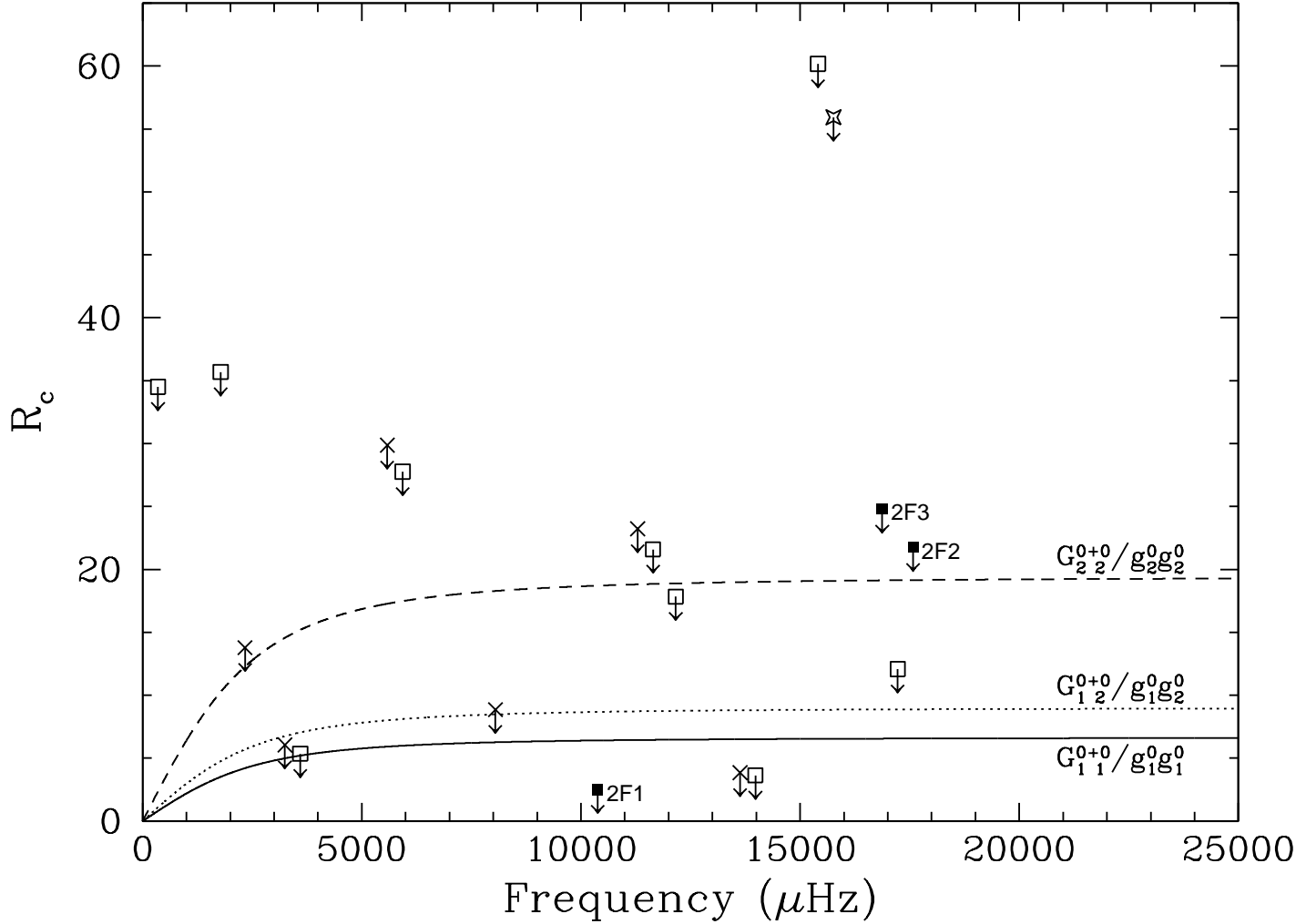
Fig. 18.— Ratio of combination to parent mode amplitudes ( R_c ) for L19-2. The lines are theoretical predictions for G_{11}^{0+0}/g_{11}^0g_1^0(\Theta_o = 16^\circ) (solid line), G_{12}^{0+0}/g_{11}^0g_2^0(\Theta_o = 16^\circ) (dotted line), and G_{22}^{0+0}/g_2^0g_2^0(\Theta_o = 16^\circ) (dashed line). The data points are the limits on the harmonics (filled squares) and limits for the cross combinations for the presumed (Bradley 2001) \ell = 1, 1 combinations (crosses), \ell = 1, 2 combinations (open squares), and an \ell = 2, 2 combination (star). The downward arrows on the limits indicate that the points represent maximum values.
