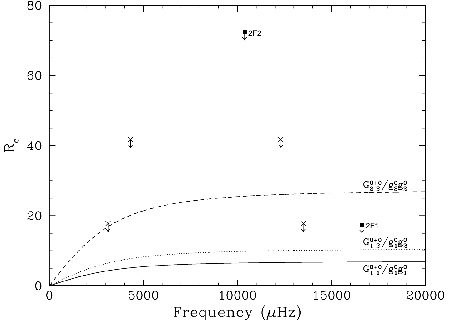
Fig. 19.— Ratio of combination to parent mode amplitudes ( R_c ) for GD 165. The lines are theoretical predictions for G_{11}^{0+0}/g_{11}^0g_1^0(\Theta_o = 25^\circ) (solid line), G_{12}^{0+0}/g_{11}^0g_2^0(\Theta_o = 25^\circ) (dotted line), and G_{22}^{0+0}/g_{22}^0g_2^0(\Theta_o = 25^\circ) (dashed line). The data points are the limits on the harmonics (filled squares) and limits for the cross combinations (crosses). The downward arrows on the limits indicate that the points represent maximum values.
