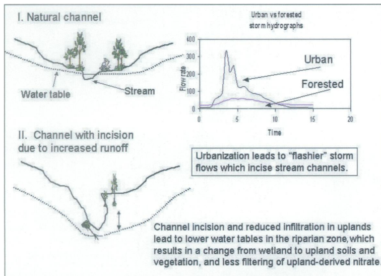
Figure 3. Conceptual diagram showing streams and associated riparian zones in forested and urban watersheds. High runoff during storms leads to incised stream channels in urban watersheds, which, in combination with reduced infiltration in impervious urban uplands, can lead to reduced riparian groundwater levels.
