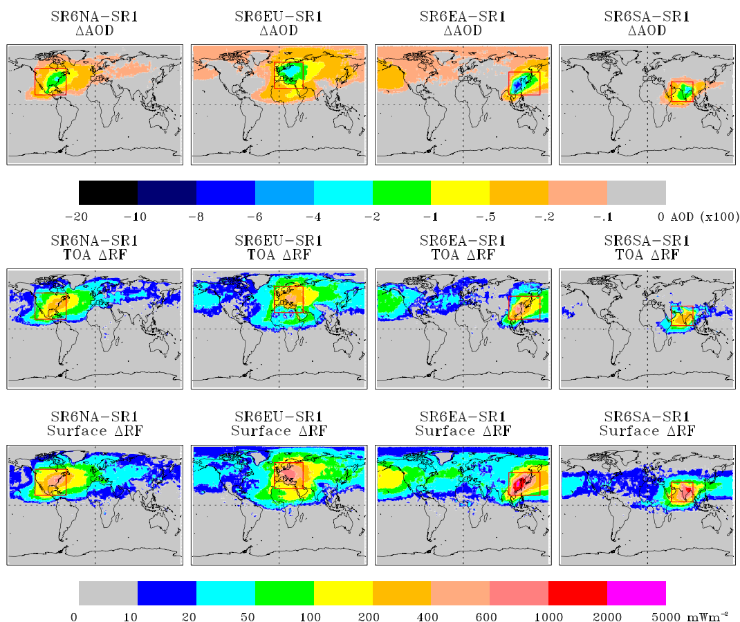
Figure 9. Annual average AOD ( \times 100 , top panel) and DRF ( \text{mW m}^{-2} ) at the top of atmosphere (TOA) (middle panel) and at the surface (bottom panel) in all-sky conditions resulting from 20% reductions of anthropogenic emissions from each region (mean of eight models). A positive value for DRF represents the reduced aerosol direct radiative forcing resulting from the reduction of emissions. Red boxes show each of the four source regions. Individual aerosol components are assumed to be mixed externally.
