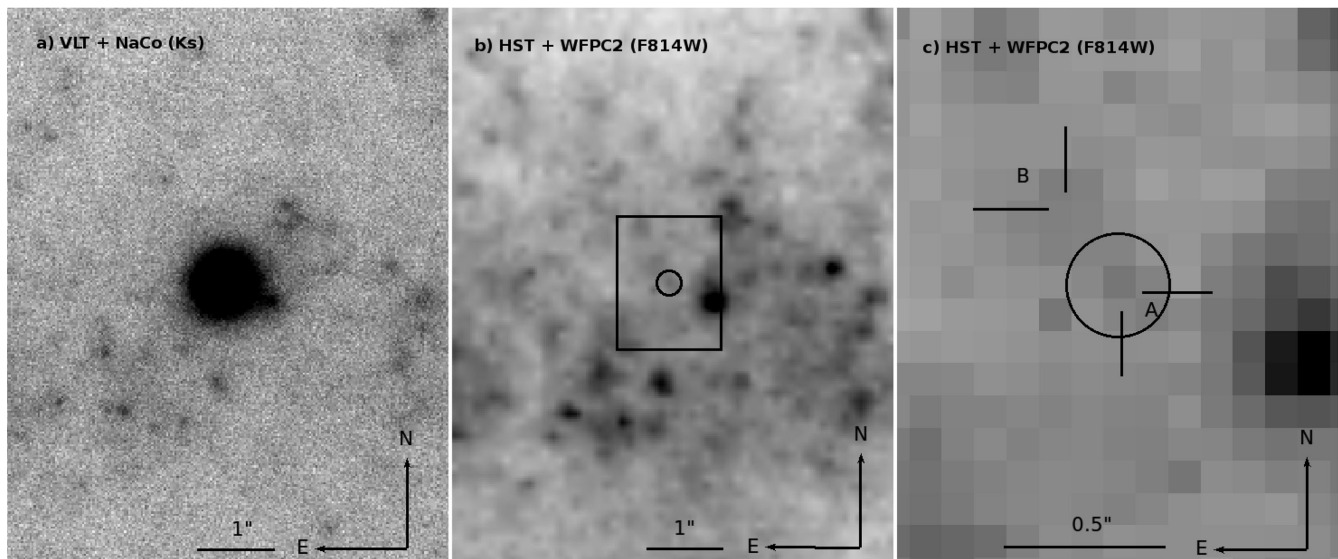
Figure 12. (a) The post-explosion image taken with VLT+NaCo 15 d after the explosion. (b) A pre-explosion image taken by HST /WFPC2 with the filter F814W. The scale and orientation of the images (a) and (b) are the same. The circle on (b) shows the position of the SN with 1\sigma uncertainty. The area marked with a square is enlarged in (c). The circle in (c) also shows the position of the progenitor, while A and B marks the sources detected with DOLPHOT (see the text and Table 6).
