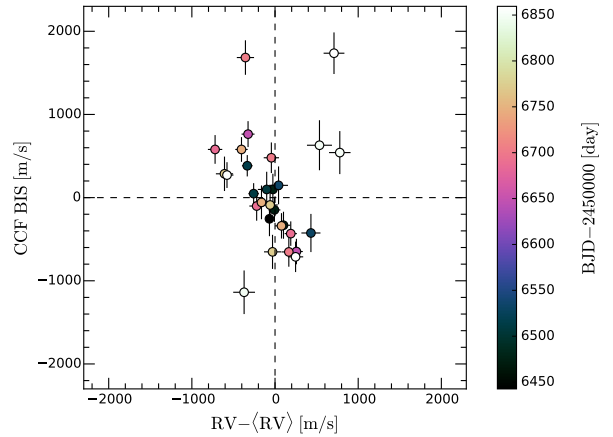
Figure 6. CORALIE measurements showing the span in the slope of the bisector plotted against the measured RV. Both quantities are anti-correlated, implying that the apparent RV variability is caused by a change in the shape of the cross-correlation function, implying that variation in the shapes of the lines are due to stellar activity.
