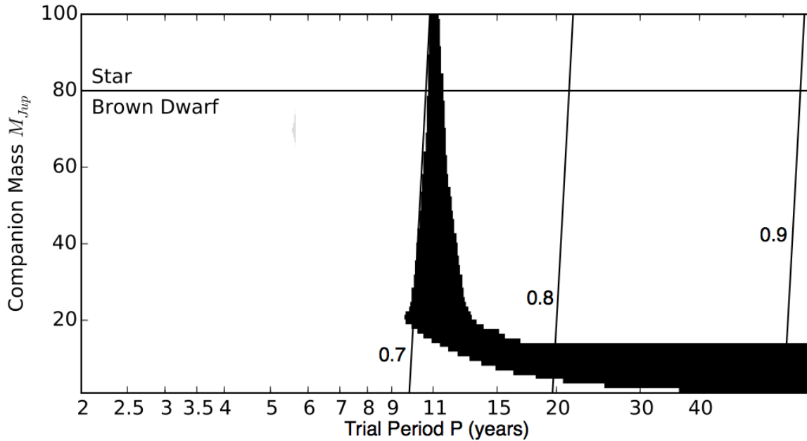
Figure 15. Combined mass-period limits for J1407b with elliptical orbits. This figure is a logical combination of the panels (b), (c) and (d) in Figure 14. Vertical lines represent ellipticities of 0.7, 0.8 and 0.9 from left to right respectively.
