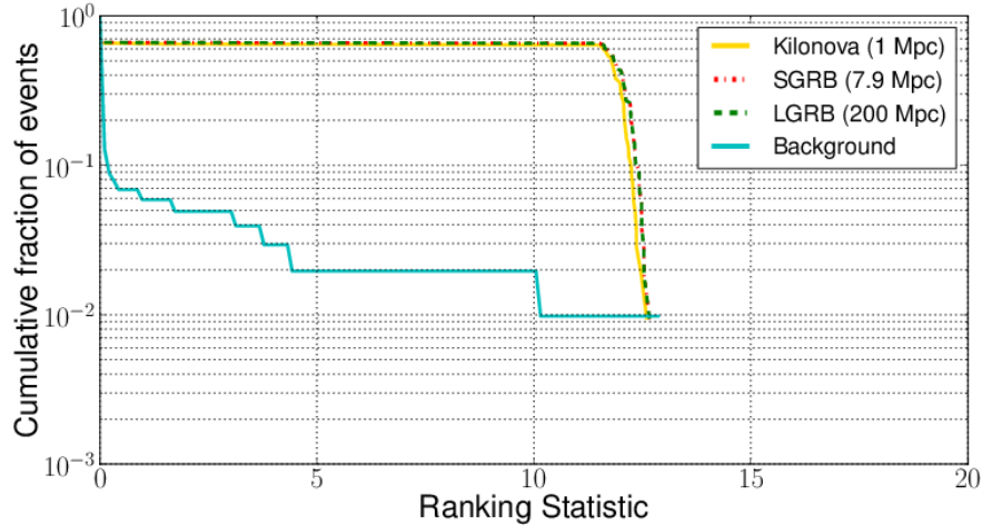
FIG. 12.— Distribution of ROTSE background (time-shifted) triggers and recovered injections for event G19377. This plot shows the distribution ranking statistic for kilonova injections simulated from 1 Mpc, short GRBs from 7.9 Mpc, and long GRBs from 200 Mpc. The GRB models correspond to the brightest observed GRB afterglows.
