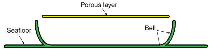
Fig. 2. The general setup of the jellyfish model. The porous layer is shown in yellow. The seafloor and main part of the jellyfish bell are shown in green and black.
