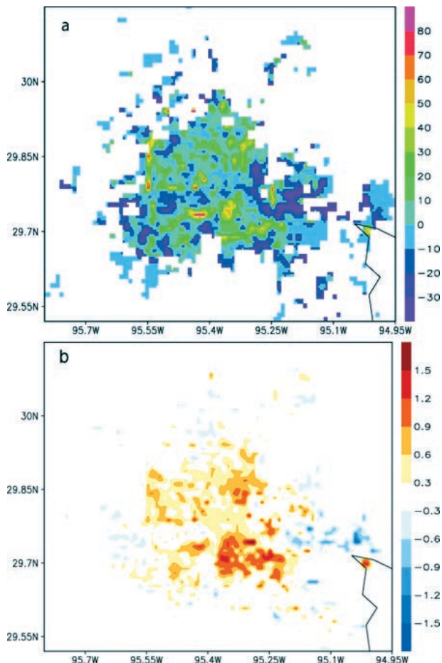
FIG. 8. (a) Difference of daily mean AH rate ( \text{W m}^{-2} ) for Houston: WRF/UCM lookup table—NUDAPT data; (b) 2-m air temperature differences (K) at 1200 UTC 30 Aug 2000 between the WRF simulation that used WRF/UCM table-based AH rate and the simulation that used NUDAPT anthropogenic heating rate.
