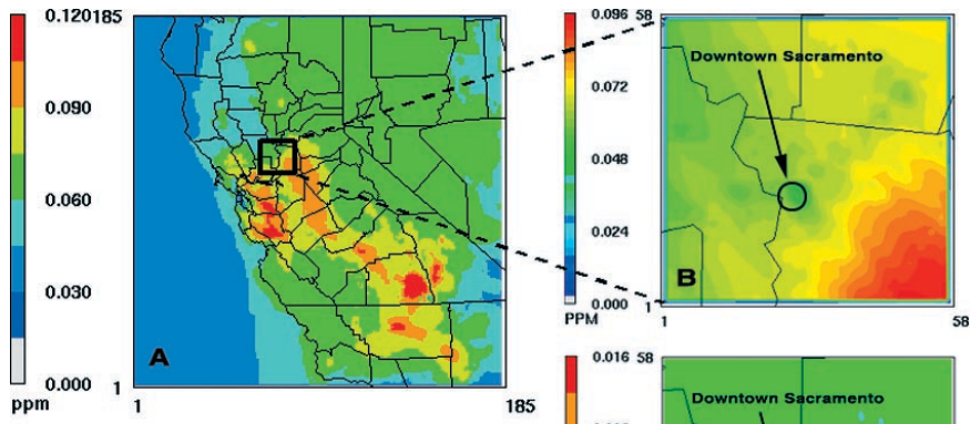
FIG. 10. Sensitivity of air quality (ozone) to UHI reduction scenario described in Fig. 9 (Taha 2008a,c). (a) Simulated base-case ozone ( \text{O}_3 ), ppm, for central California, 31 Jul 2000 (1300 PDT) at 4-km resolution. (b) The 1-km-resolution detail of simulated base-case ozone ( \text{O}_3 ) at 1300 PDT 31 Jul 2000 within the uMM5 grid for the Sacramento area. The approximate location of the area with high-rise buildings is shown with black ellipse. (c) Changes in ozone concentrations (ppm) as a result of UHI control via increased urban albedo in the Sacramento area.
