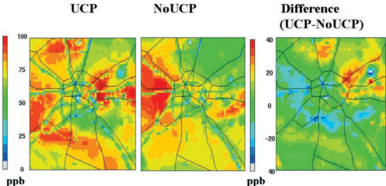
Fig. 7. Example results of ozone simulations based on CMAQ model driven by urbanized (UCP) versus standard version (no UCP) of MM5 at 1-km grid size for Houston, TX, at 2100 UTC 30 Aug 2000.
