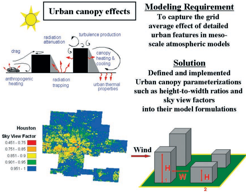
FIG. 1. Schematic of urban canopy parameterization concept and methodology. Here, sky-view factor is the ratio of the radiation received in the street canyon to the hemispheric radiation above the canopy.
