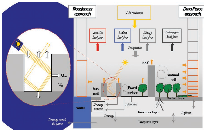
FIG. 3. Schematic showing the urbanized version of MM5 based on (drag approach) DA-SM2U (Dupont et al. 2004). Drag force approach is used in contrast to the standard roughness approach. (left) Street canyon radiative fluxes are included, and a land surface model (SM2U) provides for within-grid variations of fluxes.
