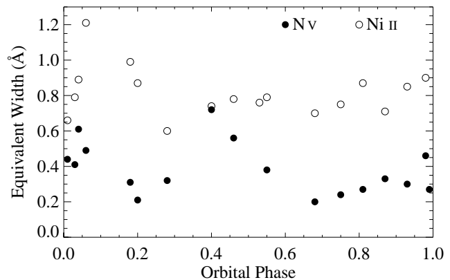
Figure 10. Equivalent widths of the N v (1242.80 Å) and Ni II (1454.84 Å) absorption lines, from the 1989 IUE data. The solid circles are for N v and the open circles are for Ni II.
