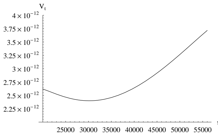
Figure 2: Total effective potential plotted for the volume range where the discriminant \Delta > 0 . For our particular choice of flux and brane numbers, the volume is stabilized at a large value \mathcal{V}_{min} \sim 3 \times 10^4 (\alpha')^3 and the minimum is de Sitter, given by V_{dS} \sim 2.4 \times 10^{-12} .
