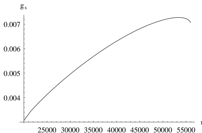
Figure 3: String coupling as a function of stabilized volume plotted in the range where \Delta > 0 .
