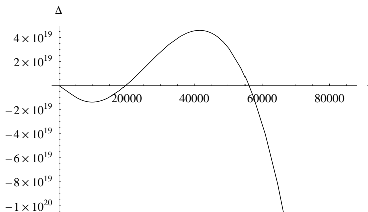
Figure 1: Discriminant (3.15) plotted as a function of volume for the set of parameter values chosen above. This plot demonstrates the excluded volume range where \Delta < 0 . The discriminant eventually again turns positive as we go to extremely large values of \mathcal{V} which are not included in this plot.
