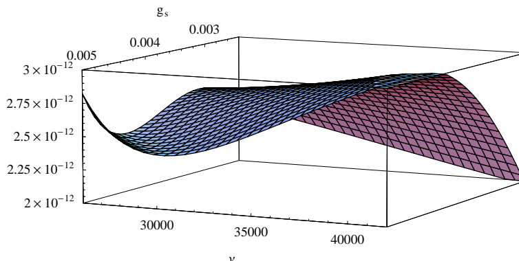
Figure 4: Effective potential (3.13) plotted as a function of string coupling and volume. The values that the volume and the string coupling can take are not restricted. The metastable de Sitter vacuum can be tuned to a desired value by discretely varying flux, topological and brane numbers.
