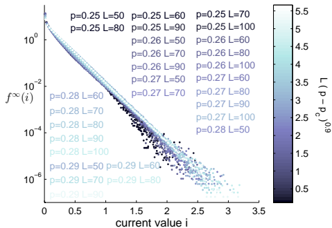
FIG. 3.4. (Color Online) Limiting current distributions f^\infty(i) = L^{-1}f_L(L^{-1}i) at different system sizes and bond densities. Colors represent the ratio L/(p - p_c)^{-0.9} where p_c \doteq 0.2488 is the percolation threshold for an infinite system and thus the color serves as an indicator of the system size relative to the correlation length. The overlap of current distributions at different parameters demonstrates a robust exponential distribution for large currents.
