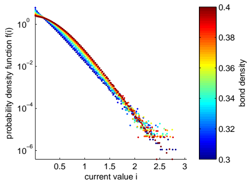
FIG. A.2. (Color online) Limiting current distributions at bond density ranging from p = .3 - .4 .
