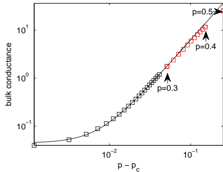
FIG. A.1. Scaling of the bulk conductance with respect to the bond density p in an 100 \times 100 \times 100 cubic lattice.
