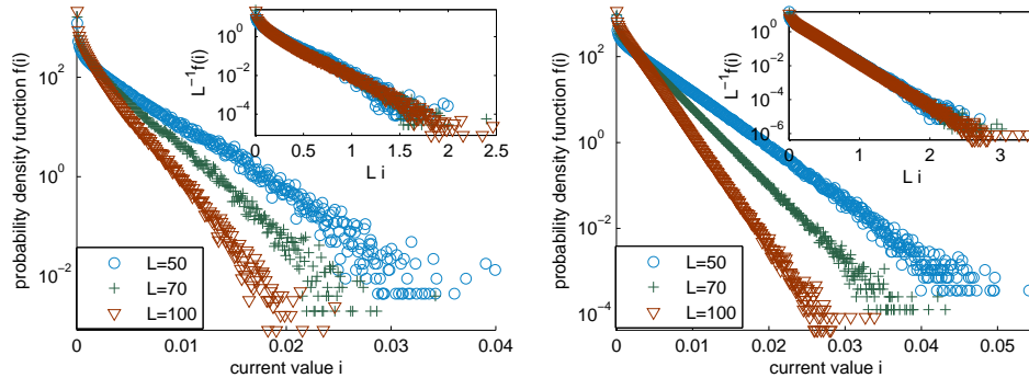
FIG. 3.2. (Color online) Empirical probability density function of the current in an L \times L \times L cubic lattice at bond density 0.25 (left) and at bond density 0.29 (right) for various system sizes L . The percolation threshold is at bond density 0.2488. A constant unit voltage is imposed across the system. The plot is derived from the histograms of all the currents over 1000 realizations. The inset shows the same distributions rescaled by the system L with critical exponents u = 1 and v = 1 .
