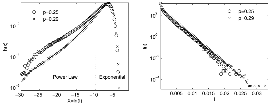
FIG. 3.1. Distribution h(x) of the logarithmic current (left) and distribution f(i) of the current (right) near threshold ( p = 0.25 ) and above threshold ( p = 0.29 ) in 100 \times 100 \times 100 random resistor networks. The logarithmic transformation of currents exposes small currents which have a power law distribution (left panel) while the overall current distribution looks exponential (right panel).
