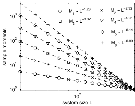
FIG. 3.3. Scaling of the first 6 sample moments with respect to the system size L . The bond density is fixed at p = 0.25 and the system size L varies from 50 to 200. The fitted equations of the moments M_k are shown in the figure (cf. Equation (3.3)). Curves are normalized by their values at L = 200 .
