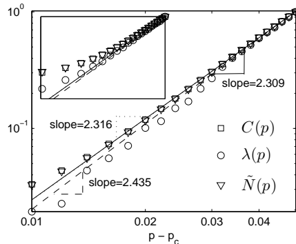
FIG. 3.5. Scaling behaviors against bond density p - p_c^{\text{eff}} for the bulk conductance C(p) , the rate \lambda(p) of the exponential tail of the current distribution, and the number \tilde{N}(p) of bonds with current larger than 10^{-3} . The system size is fixed at L = 100 and the bond density p varies from 0.25 to 0.29. Curves are normalized by their values at p = 0.29 . In the parent figure p_c^{\text{eff}} = 0.24 as defined in [35] and p_c^{\text{eff}} = 0.2488 in the inset. The inset demonstrates the sensitivity of the scaling exponent on the value of p_c used (with fitted exponents 1.919 \pm .012 , 1.969 \pm .077 and 1.917 \pm .013 respectively), but further supports the similar behavior of \lambda(p) and C(p) .
