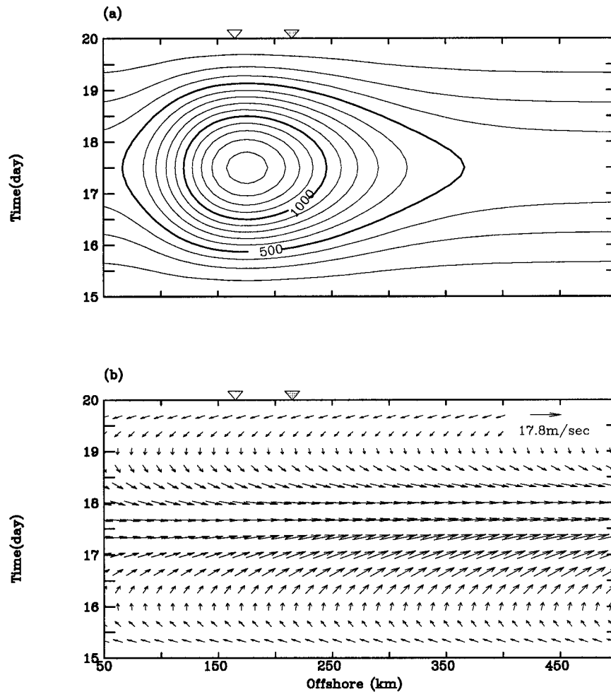
FIG. 6. Total heat flux (a) and the wind (b) imposed on the sea surface in the model to simulate atmospheric forcing during a severe winter storm [adapted from Xue et al. (1995)].
