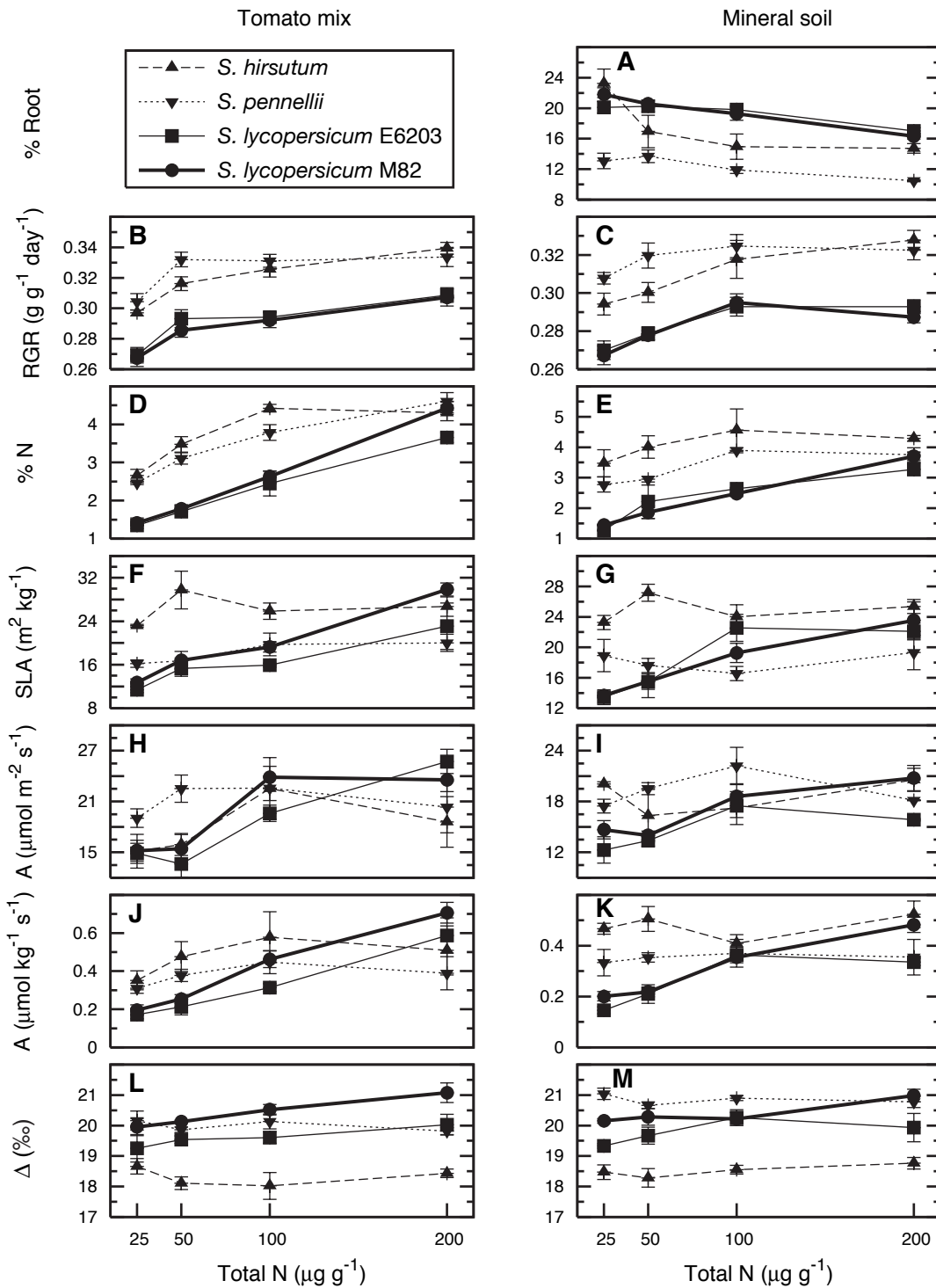
Fig. 2. Effects of nutrient level and soil media on tomato. Two potting media were tested factorially with the nutrient levels, 1) a mineral soil (panels A, C, E, G, I, K, M) and 2) a standard vermiculite/peat based soil: 'tomato-mix' (panels B, D, F, H, J, L). Shown are percent root, calculated on soil-washing in the mineral soil only and representing all size classes of roots (A), the relative growth rates (B, C), %N measured for leaf-blade tissue only (D, E), leaf area per unit leaf mass (F, G), photosynthetic carbon assimilation per unit leaf area per second (H, I), the same carbon assimilation expressed as a rate per unit leaf mass per second (J, K), and \Delta (L, M). Each datapoint represents the mean of six replicate plants for %root, RGR, %N, and \Delta , and 4 plants for SLA and A. Error bars are \pm one SE. Wild species relatives are also distinguished from tomato cultivars by dashed and solid lines, respectively.
