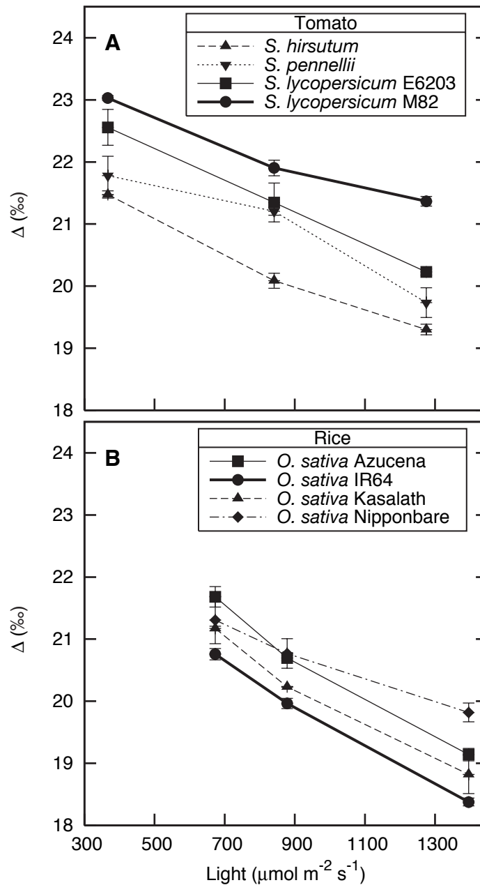
Fig. 6. Effects of growth irradiance on \Delta in selected tomato (A) and rice (B) genotypes. All plants were grown together in a glasshouse but received varying degrees of supplemental HID lamp output. Light levels given are mean photoperiod irradiances of total PAR. Datapoints represent the means of six replicate plants, and error bars are \pm one SE.
