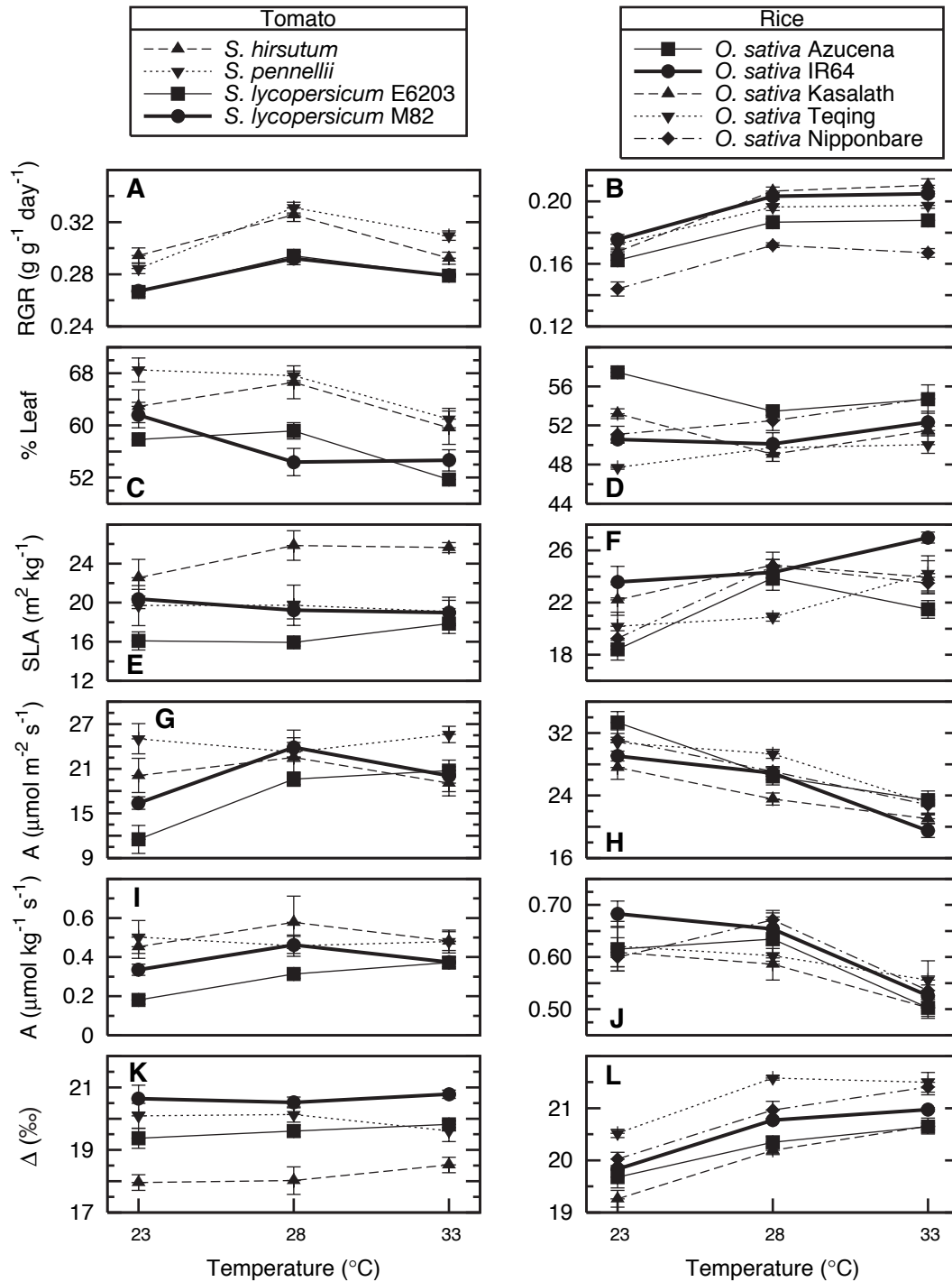
Fig. 1. Effects of variation in mean growth temperature during the photoperiod for a selection of both tomato (panels A, C, E, G, I, K) and rice (panels B, D, F, H, J, L) genotypes. These panels represent half of the data (one soil media) dealt with in factorial design in Tables 2 & 3. Shown are the relative growth rates (A, B), per cent of shoot biomass allocated to leaf blade tissues (C, D), leaf area per unit leaf mass (E, F), Photosynthetic carbon assimilation per unit leaf area per second (G, H), the same carbon assimilation rate expressed per unit leaf mass per second (I, J), and carbon isotope discrimination (K, L). Each data point represents six plants for RGR, percent leaf, and \Delta . Four plants for SLA and A. Error bars show \pm one SE. Plot symbols represent different genotypes. In tomato panels wild species relatives are also distinguished from tomato cultivars by dashed and solid lines, respectively. In rice panels, line dashing is a visual aid but follows no specific pattern.
