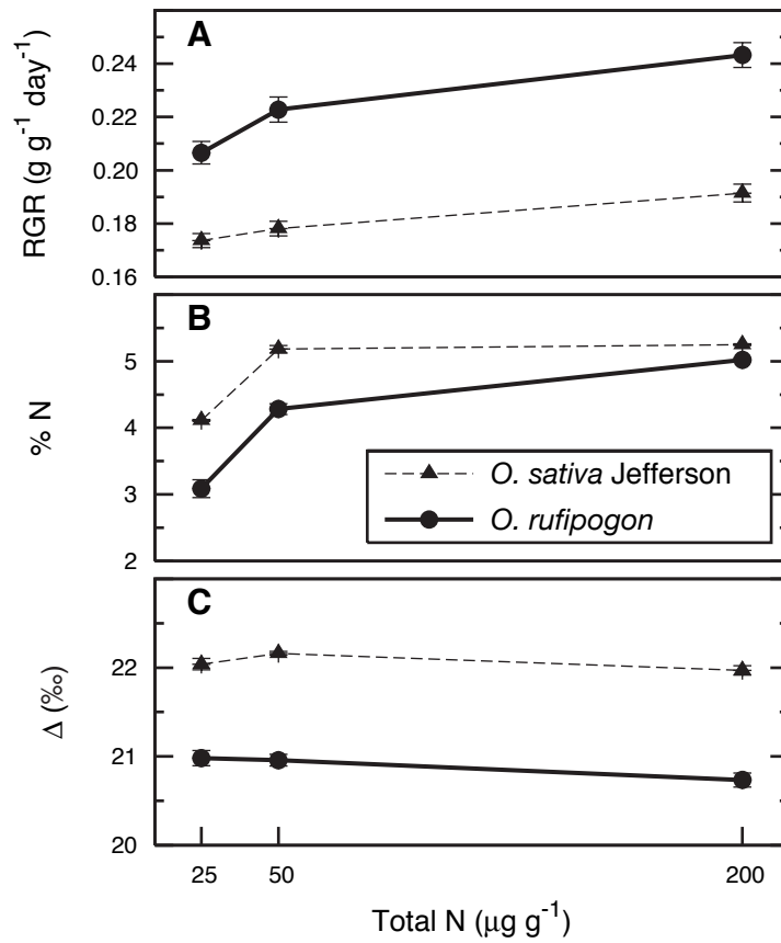
Fig. 3. Response of two rice genotypes to nitrogen concentrations. A) the whole plant relative growth rates, B) %N measured for leaf-blade tissue only and C) carbon isotope discrimination. Each datapoint represents the mean of six replicate plants. Error bars are \pm one SE.
