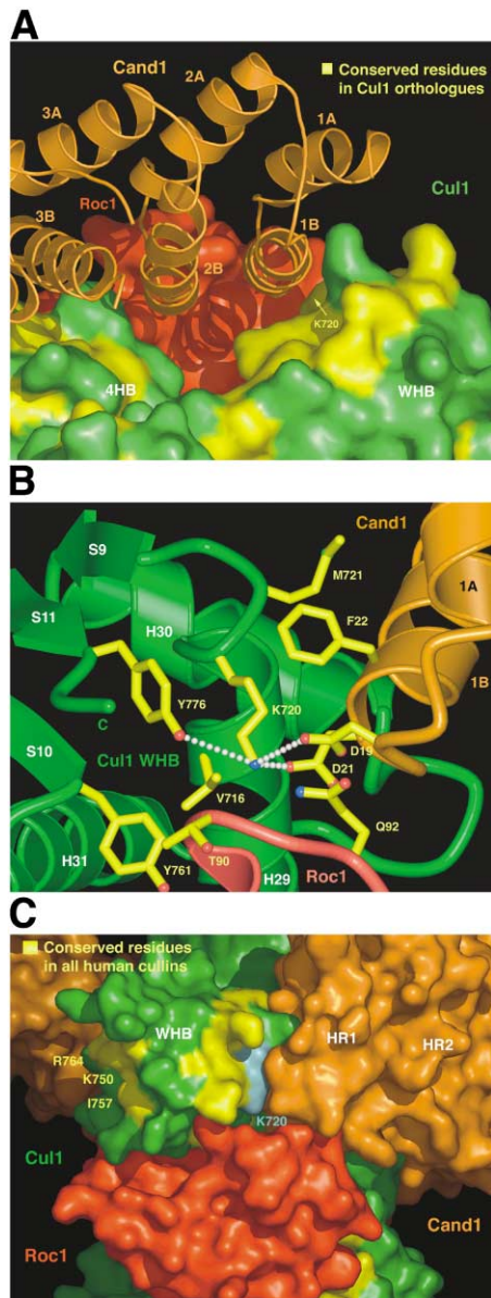
Figure 5. The N-terminal HEAT Repeats of Cand1 Interact with a Conserved Surface Cleft of the Cul1 CTD and Bury the Cul1 Neddylat-ion Site Lysine Residue
