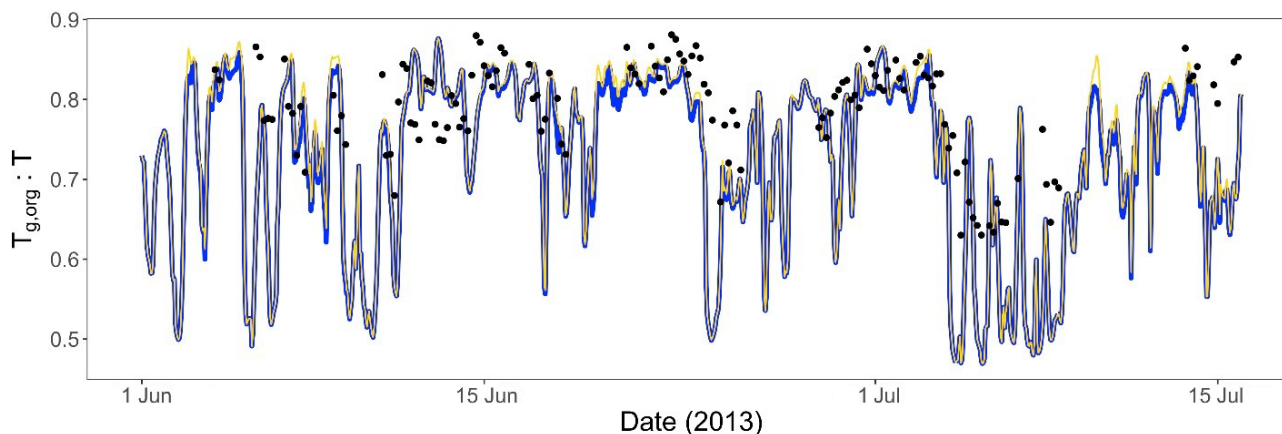
Figure 5. Predicted glass transition temperature to ambient temperature ratio ( T_{g,\text{org}} : T ) at the Centreville, AL, site during the 2013 SOAS campaign based on OA composition reported by H. Zhang et al. (2018) (black). Predicted T_{g,\text{org}} : T from this work is shown in blue for PhaseSep and gold for PhaseSep2.
