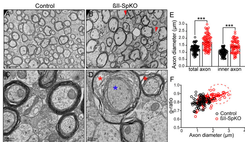
Fig. 2. \beta II-spectrin maintains the caliber and integrity of myelinated CC axons. ( A and B ) TEM images of cross-sections through the CC from \beta II-Sp fllox/flox +/+ ( A , control) and \beta II-Sp fllox/flox /Nestin-Cre ( B , \beta II-SpKO) PND25 mice ( n = 3 mice). Red arrowheads indicate inflammatory microglia. (Scale bars, 2 \mu m.) ( C and D ) Higher-magnification images of CC axons from control ( C ) and \beta II-SpKO ( D ) mice. Asterisks indicate degenerating axons with decompaction of the myelin sheath and vacuolization (red asterisks) and debris (blue asterisk). (Scale bars, 200 nm.) ( E ) Comparison of myelinated axon diameter from control ( n = 85 ) and \beta II-SpKO ( n = 84 ) CC axons. Data represent mean \pm SEM. Student's t test, *** P < 0.001 . ( F ) g-ratio versus axon diameter from CC of PND25 control and \beta II-SpKO mice. Red dotted circle area represents a population of \beta II-SpKO large-diameter axons with decreased myelin content that is absent in control brains.
