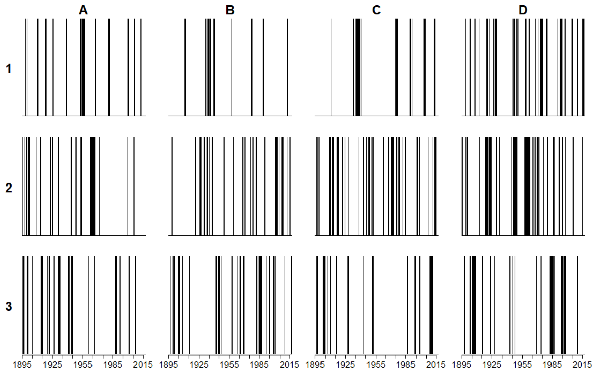
Figure 2. For each cartographic visualization (Fig. 1) a corresponding absence and presence bar plot was generated to visually characterize both the return periods and persistence (duration) of patterns from 1895-2016. Thicker bands represent longer persistence.
