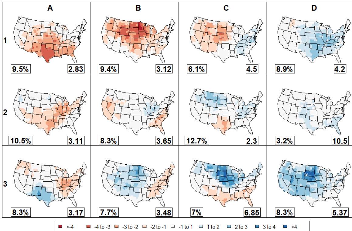
Figure 1: Self-Organizing Cartographic Maps (1-12). Percentage value (lower left) indicates the percentage of total months within the study period. Values in the lower right represent persistence of trends, where higher values indicate longer durations, and lower values indicate shorter duration trends (Gibson et al. 2016).
