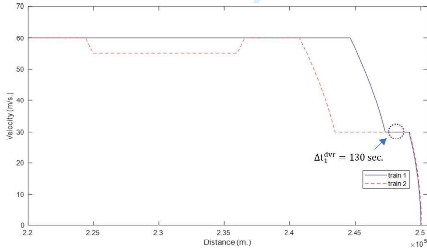
Figure 6: Velocity profile when passing a diverging junction
