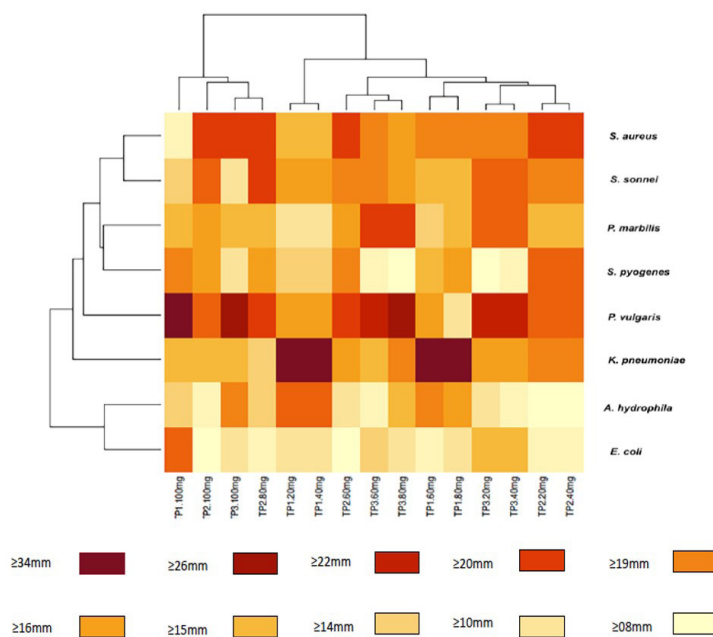
Figure 5. Heatmap showing the antimicrobial activity of different kinds of toothpaste against bacterial strain. TP1 stands for toothpaste 1 , and the TP2 stands for toothpaste 2 , TP3 stands for toothpaste 3 . The tree is a dendrogram, which shows the hierarchy (similarity) between isolates and their activity against the Oral different pathogens. The graph was plotted using the R program.
