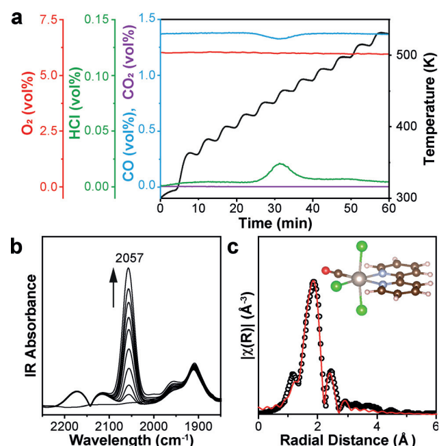
Figure 2. Evolution from [bipy-Ru III Cl 4 ] - to mer (Cl)-[bipy-Ru III (CO)Cl 3 ]. a) Mass spectrometry (MS) showing the outlet gas profile with the corresponding temperature profile under 1% CO and 5% O 2 flow, O 2 is fed to monitor if there is any oxidation of CO to CO 2 . Blue CO, purple CO 2 , red O 2 , green HCl. b) In situ DRIFTS spectra, showing the formation of one terminal CO coordination at 2057 cm -1 . c) Experimental and fitted EXAFS data, suggesting the [bipy-Ru III (CO)Cl 3 ] single-site structures with corresponding DFT calculated models.
