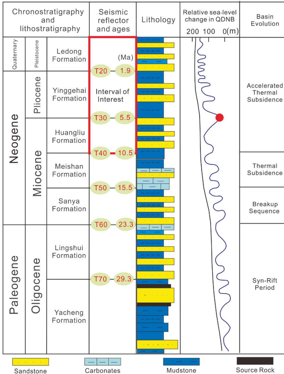
Fig. 2 Tectono-stratigraphic column of the Qiongdongnan Basin (Gong et al., 2011; Han et al., 2016; Xie et al., 2008b; Zhao et al., 2016). Relative sea-level changes in the Qiongdongnan Basin are based on Wei et al. (2001). The red rectangle indicated the interval of interest in our study. The red arrow points to the sea-level lowstand recorded at 5.5 Ma b.p.
