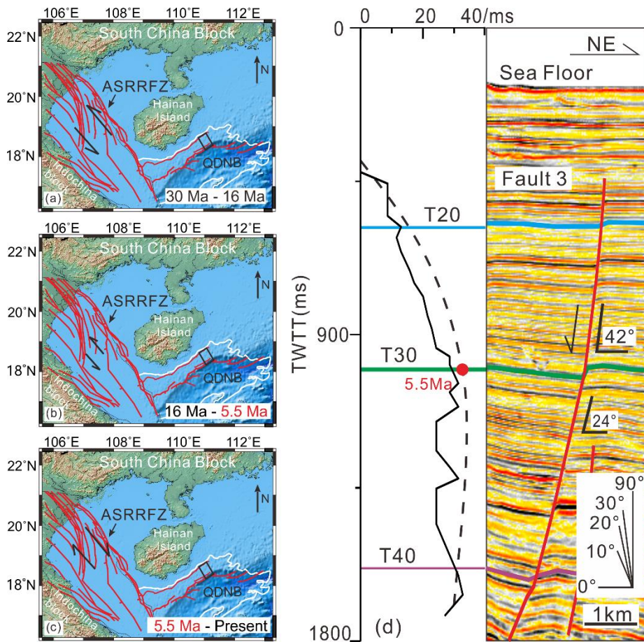
Fig. 11 Movement of the Ailao Shan-Red River Fault Zone included: (a) a predominant sinistral movement from ~ 30 to 16 Ma (b), a transitional phase between 16 and 5.5 Ma, and (c) a change to a predominant dextral movement after 5.5 Ma (Zhu et al., 2010). The black rectangle shows the location of the study area. (d) T-z plot of Fault 3 documenting the effect of slip reversal in the Ailao Shan-Red River Fault Zone at 5.5 Ma (T30). The dotted line represents the trend of the T-z plot according to the K value, and the red point indicates the reversal in the gradients of the T-z plot. The blue, green and purple lines represent horizons T20, T30 and T40 respectively. Abbreviations: QDNB= Qiongdongnan Basin; HI= Hainan Island; ASRRFZ= Ailao Shan-Red River Fault Zone.
