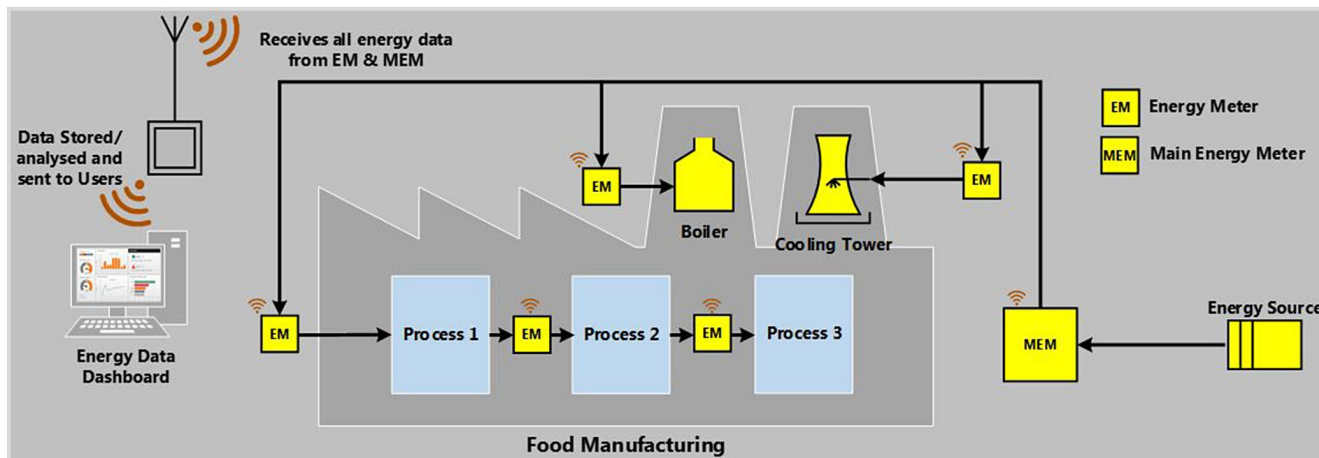
FIGURE 3 Energy monitoring system
