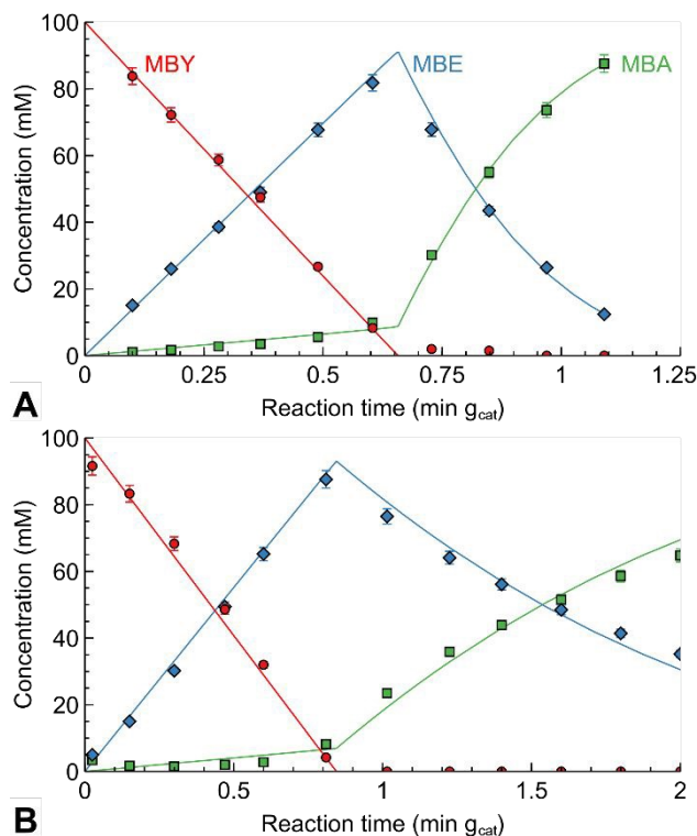
Figure 4. Concentration profile of MBY semi-hydrogenation over (A) the original and (B) Pb-poisoned 2 wt% Pd/CaCO 3 catalyst with the lines corresponding to the model fit.
