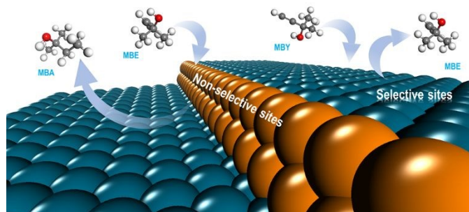
Figure 8. Scheme of the selective (terrace) and non-selective (low-coordination) sites on the Pd catalysts for alkyne semihydrogenation.
