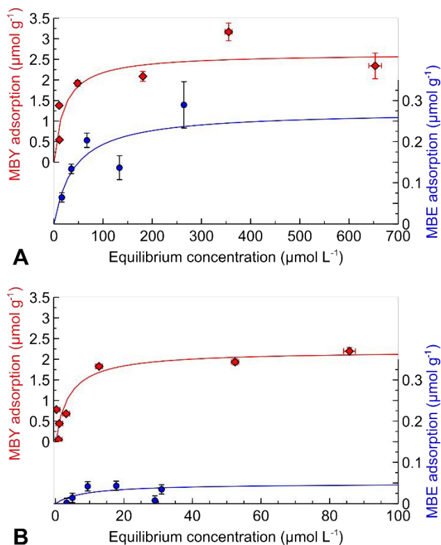
Figure 2. Adsorption isotherms of individual species, MBY and MBE, over the (A) 2 wt% Pd/CaCO 3 and (B) Pb-poisoned 2 wt% Pd/CaCO 3 catalysts.
