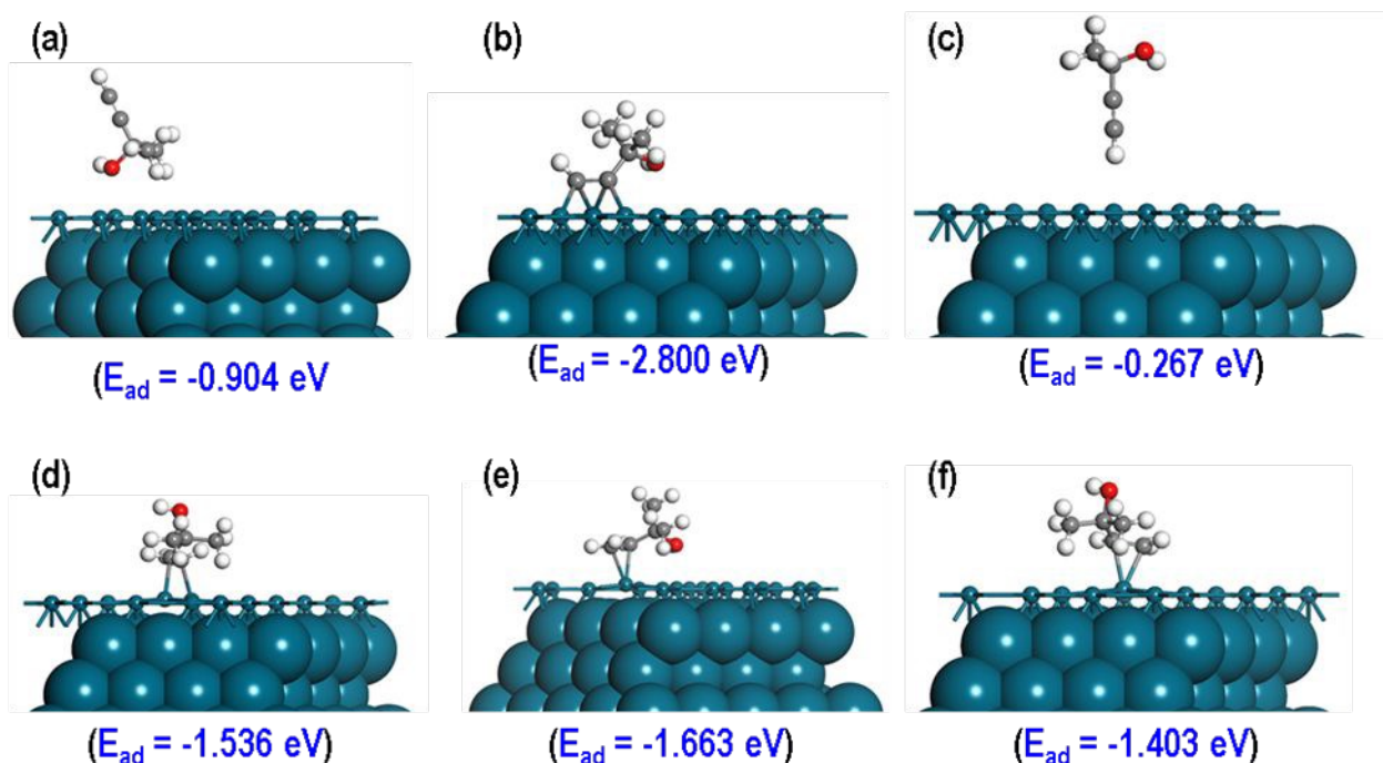
Figure 5. Most stable structures of MBY adsorbed (a) via H atom, (b) over the O atom, (c) via CH group, and MBE adsorption (d) via H atom, (e) via OH group, (f) via \text{CH}_3 group. The top layer of Pd(111) surface along with the adsorbed molecule shown in ball and stick representation for clarity.
