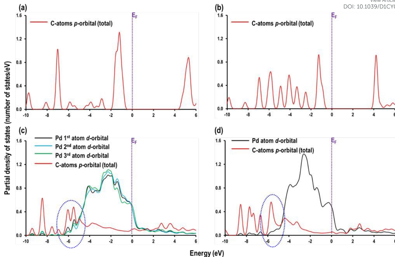
Figure 6. Partial density of states for (a) MBY and (b) MBE molecules in gas phase, and (c) MBY and (d) MBE molecules adsorbed on the Pd (111) surface. The Fermi energy ( E_F ) is a dotted line at 0 eV.
