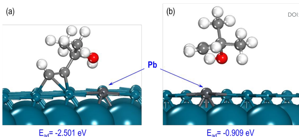
Figure 7. Optimised structures of (a) MBY and (b) MBE molecules on Pd(111) surface doped with 1 Pb atom.
