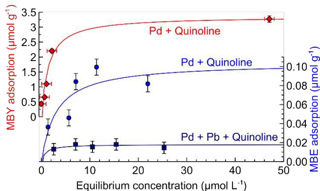
Figure 3. Adsorption of MBY or MBE over the Pd catalyst and MBE over Pd-Pb, all with pre-adsorbed quinoline at an equilibrium concentration of 8 \mu\text{mol L}^{-1} .
