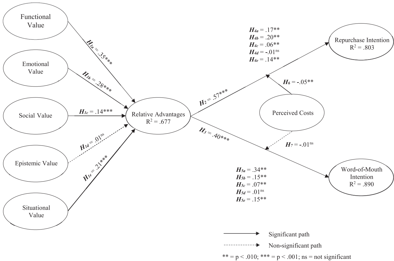
Fig. 3. . Estimation results for the structural model.
