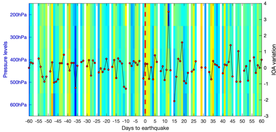
Fig. 8. Temporal variations of IOV at different pressure levels in troposphere and IOA over the epicentral region 60 d prior and after the Jiuzhaigou earthquake. Black line shows IOA variations. Red dash line indicates the day of earthquake event.
