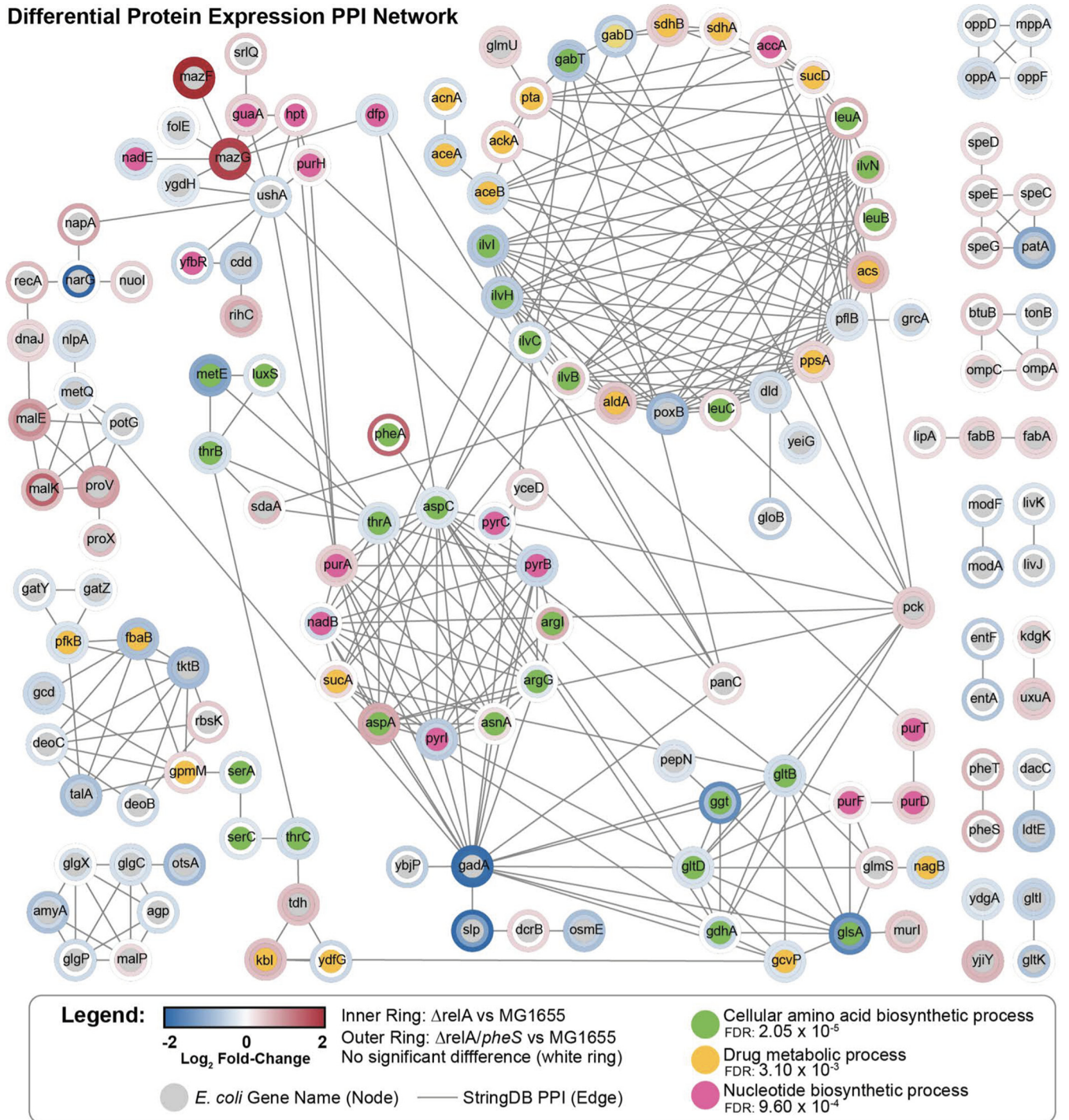
FIG 3 Protein homeostasis is disrupted during bacterial antibiotic persistence. Differential protein expression protein-protein interaction (PPI) network was performed for wild-type pheS/pheT and pheS A294S in relA + and \Delta relA backgrounds grown in medium B. The differentially expressed proteins are represented by their fold change for either \Delta relA wild-type pheS/pheT versus relA + wild-type pheS/pheT (inner ring) or \Delta relA pheS A294S versus relA + wild-type pheS/pheT (outer ring). The E. coli gene name is shown in the node, and cellular processes for amino acid biosynthesis (green), drug metabolism (yellow), and nucleotide biosynthesis (pink) are highlighted. Edges are derived from previously determined protein-protein interactions within StringDB.
