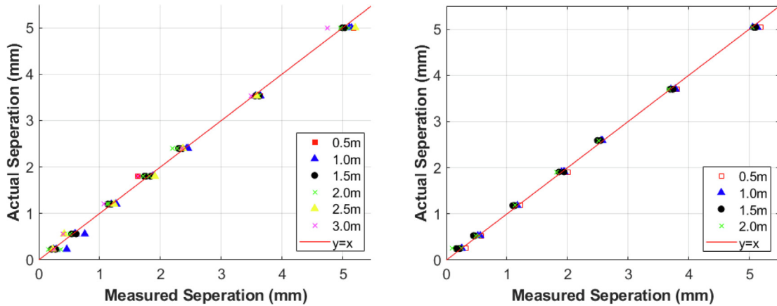
Fig. 8. Comparison of the measured vs actual separation of the brick blocks; tape markers (left), and the paint markers (right).
