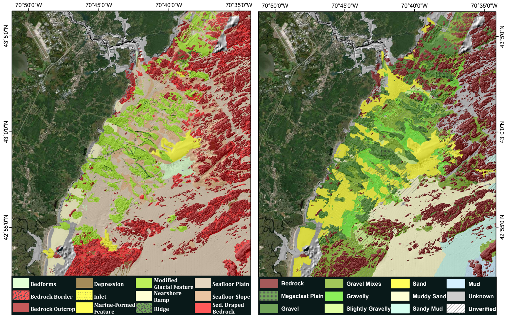
Figure 2-3. Surficial Geology of the inner continental shelf off the coast of NH (modified from Ward et al., 2021a). The major geoforms (or physiographic features) are shown on the left and the surficial sediments classification (based on CMECS) is shown on the right. The nearshore shelf within ~10 km of the NH coast is composed of: extensive megaclast platforms, many of which extend offshore from the headlands along the coast; sandy nearshore ramps which extend from the beaches; bedrock outcrops offshore and along the coast; and extensive seafloor plains composed of sand, gravel mixes, and gravel.
