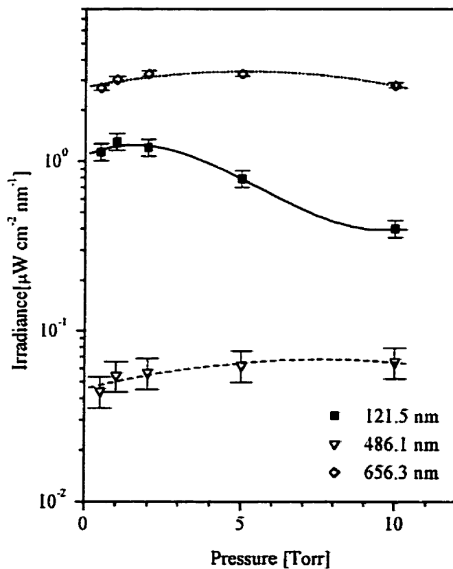
Figure 3.7 Pressure dependence of atomic hydrogen lines for H 2 -Ar mixture; P = 250 W, \Phi = 100 sccm.
