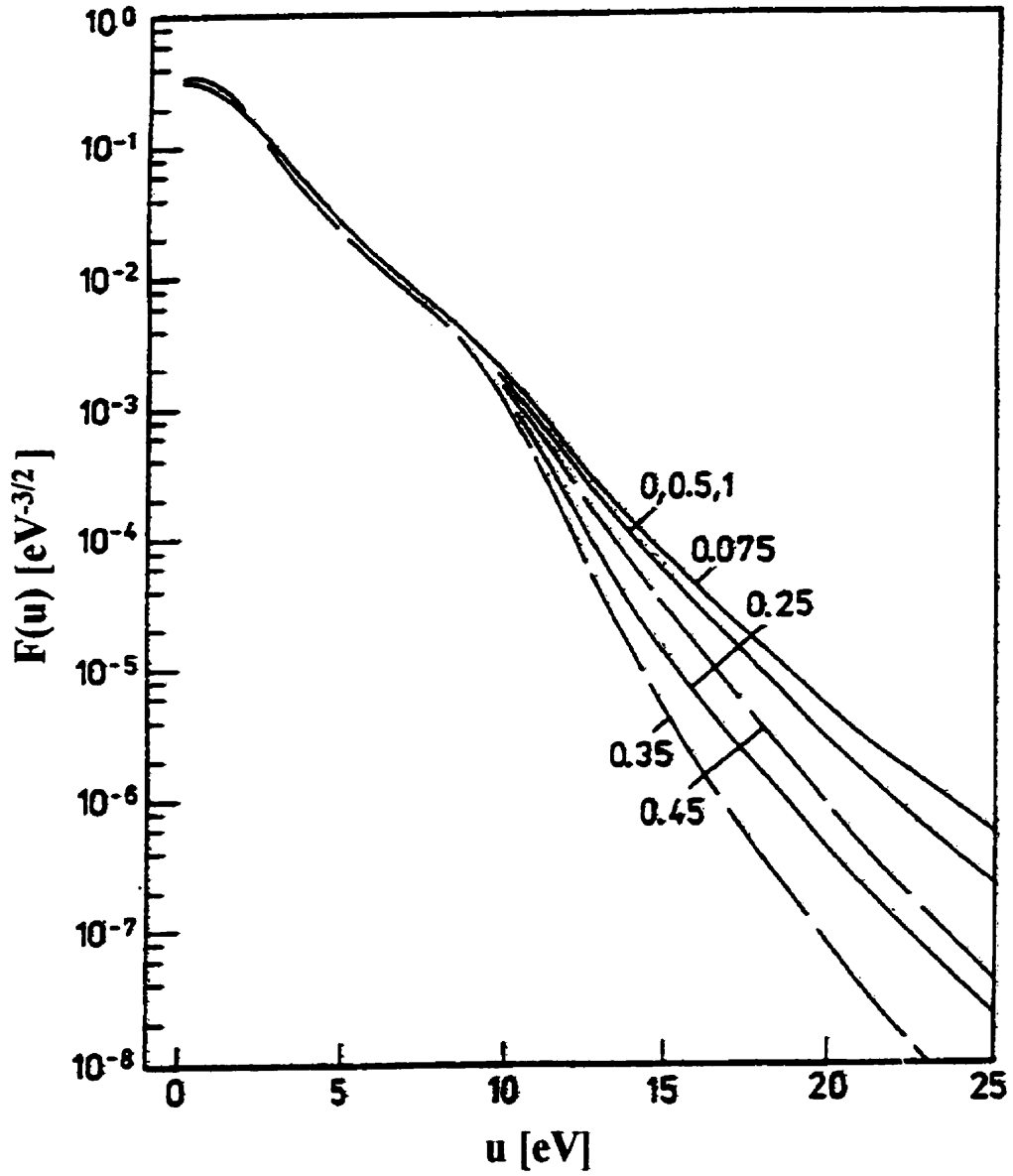
Figure 4.2 The periodic alteration of the energy distribution of electrons in \text{H}_2 plasma at a field amplitude E_0/p_0 = 23 \text{ V cm}^{-1} \text{ Torr}^{-1} and \omega/p_0 = \pi 10^8 \text{ s}^{-1} \text{ Torr}^{-1} (After Winkler et al., 31, 32 with permission).
