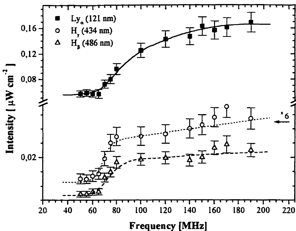
Figure 4.9 Frequency dependence of the intensities of atomic hydrogen lines for the hydrogen-argon mixture plasma ( P=25 W, p=0.5 Torr): \blacksquare Ly _{\alpha} (121.5 nm), \circ H _{\gamma} (434.1 nm), \triangle H _{\beta} (486.1 nm). The intensity of the H _{\gamma} line has been multiplied by a factor of 6.
