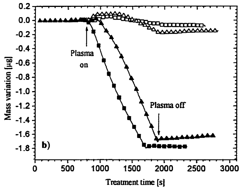
Figure 5.4 QCM response for the two sample orientations: parallel (open symbols) and perpendicular (black symbols) for: a) PE ( \square , \blacksquare ) and HTC ( \circ , \bullet ); b) PS ( \Delta , \blacktriangle ) and PE ( \square , \blacksquare ).
