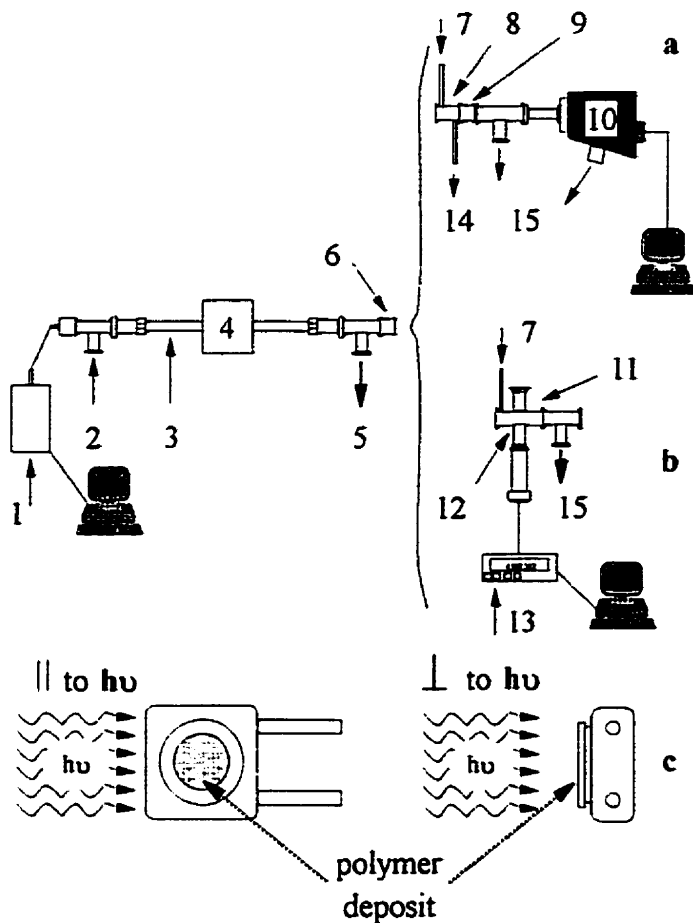
Figure 5.1 (a,b): Experimental setup: 1 - monochromator with OMA detection; 2 - gas inlet; 3 - plasma chamber; 4 - microwave cavity; 5 - mechanical pumping unit; 6, 9 - \text{MgF}_2 windows; 7 - oxygen inlet; 8 - absorption chamber; 10 - VUV monochromator; 11 - sample chamber; 12 - QCM; 13 - frequency counter; 14, 15 - turbomolecular pumping units; (c): QCM orientation with respect to the VUV photon flux ( h\nu ): parallel ( \parallel ) and perpendicular ( \perp ) to h\nu .
