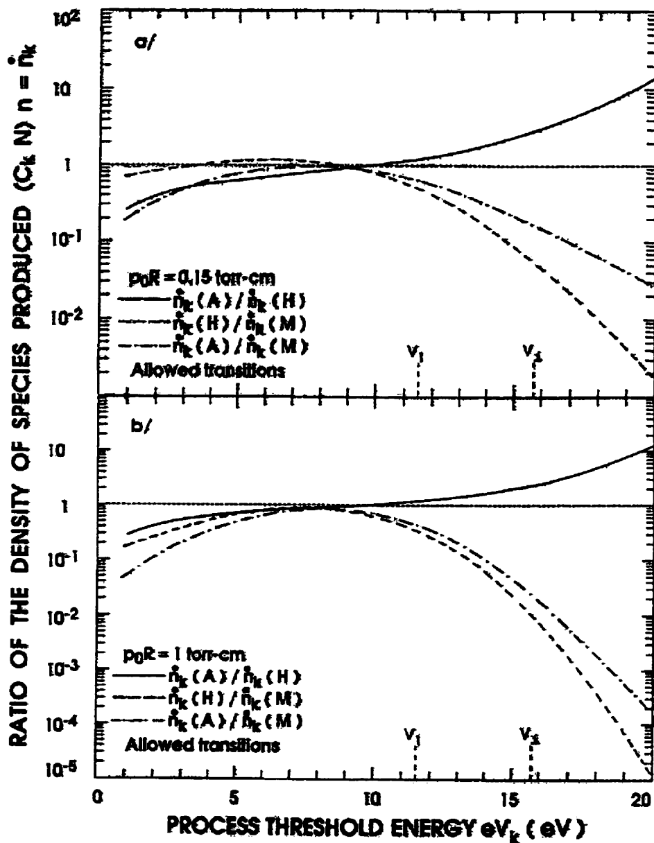
Figure 4.11 Ratios of the densities of species produced per second (C_k N) calculated with the EEDF corresponding to the three limiting situations «A» (DC), «H» (microwaves), and «M» (Maxwellian EEDF), as a function of the process threshold energy eV_k , under constant power density conditions. The process is assumed to result from electron impact on the atom (molecule) in the ground state and the cross-section used simulates an optically allowed transition. (a) p_0 R = 0.15 Torr cm, and (b) p_0 R = 1 Torr cm (after Ref. 21).
