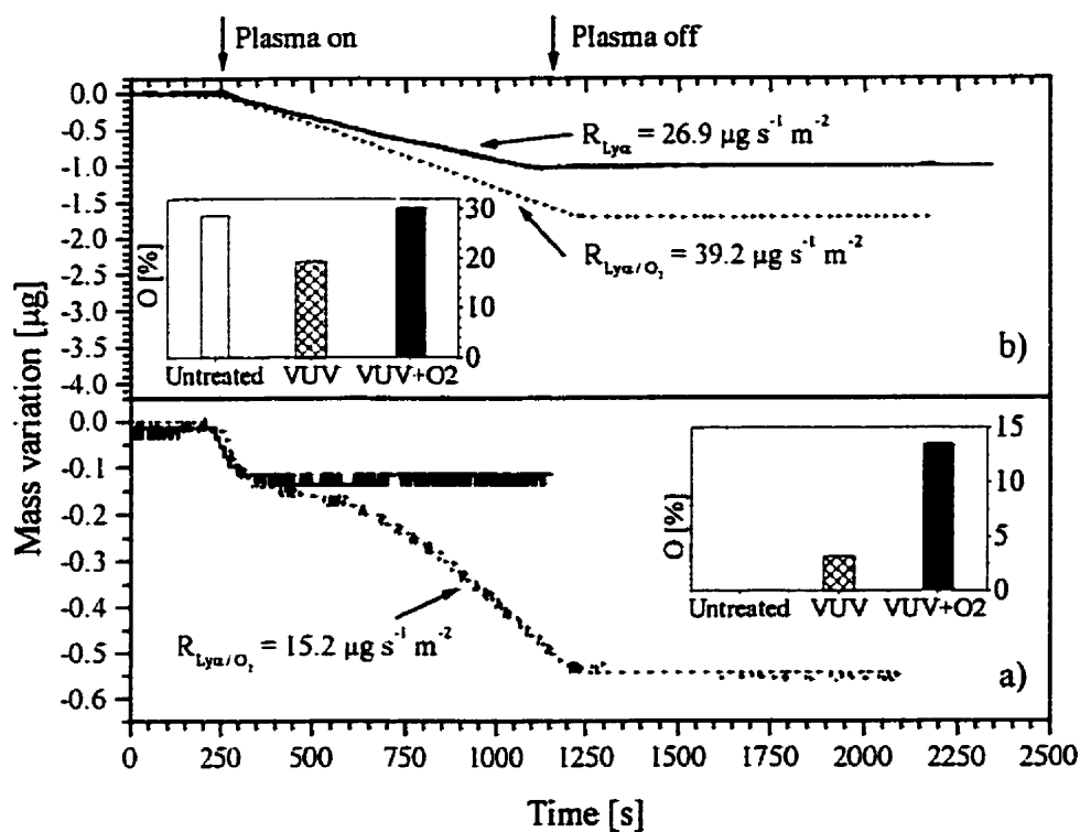
Figure 5.7 QCM response for (a) PE and (b) PMMA treated with the near-monochromatic radiation from a \text{H}_2/\text{Ar} mixture plasma: — treatment (1), - - - treatment (3). The inserts show the oxygen concentration at the sample surface (atomic percent), as measured by XPS.
