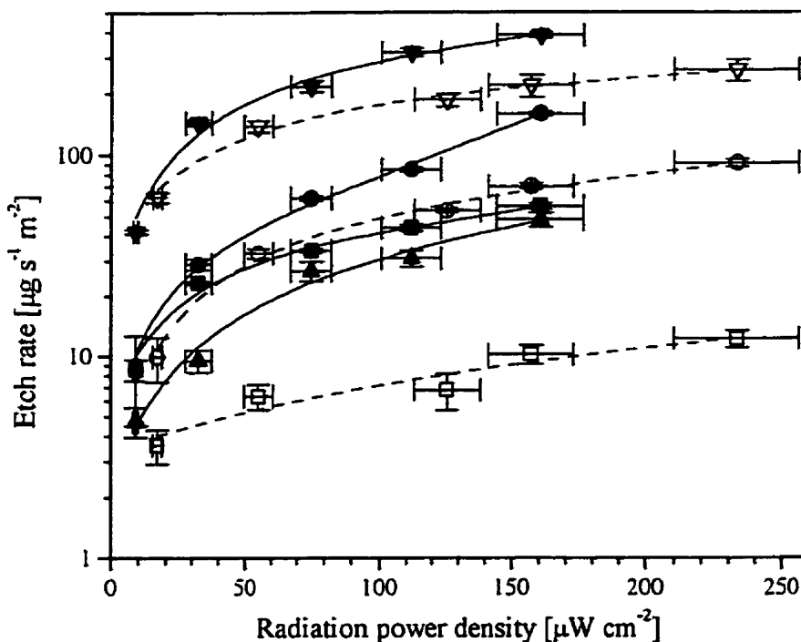
Figure 5.5 Polymer etch rate dependence on integrated VUV-UV radiation power density for samples in the perpendicular orientation: \blacksquare PE, \bullet HTC, \blacktriangle PS, \blacktriangledown PMMA. Black symbols represent VUV/AO treatment [(condition (3))]; open-strikethrough symbols represent VUV treatment in vacuum [condition (1)]; etch rate data for PS are not shown because they are too low to present here
