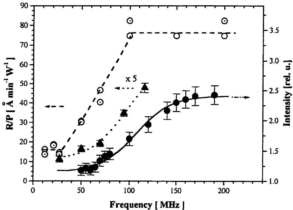
Figure 4.14 Frequency dependence of the total emission intensity in the investigated VUV region (100-200 nm), at constant absorbed power, of the hydrogen-argon mixture plasma (●) and of the deposition rate normalized to the absorbed power, R/P , for: ⊙, ○, plasma polymerized isobutylene at “low” and “high” power, respectively (after Ref. 21), and ▲ plasma enhanced chemical vapor deposition of microcrystalline silicon ( \mu\text{c:Si:H} ; after Ref. 11)
