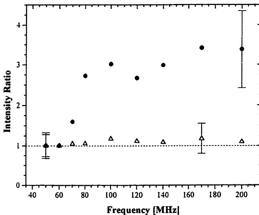
Figure 4.7 Frequency dependence, for the hydrogen plasma ( P = 50 W, p = 0.5 Torr), of the intensity ratios, normalized to the values at 50 MHz, for : ● H_{\beta} to molecular bands, Δ H_{\beta} to H_{\delta} .
