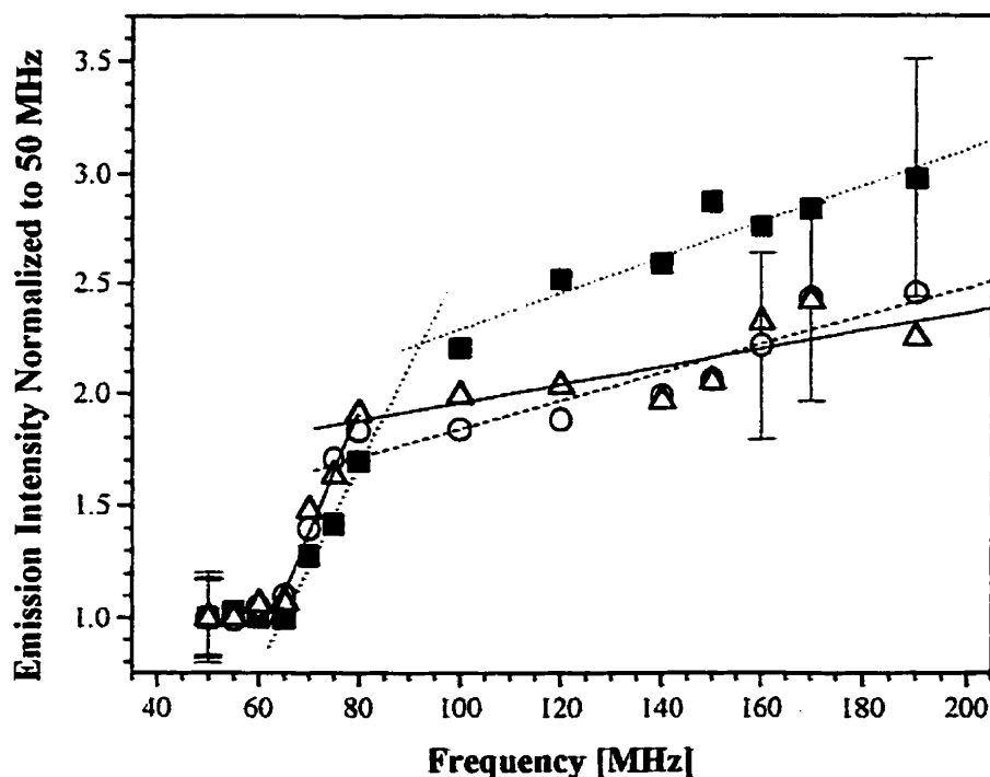
Figure 4.12 Frequency dependence, for the hydrogen-argon mixture plasma ( P=25 W, p=0.5 Torr), of the atomic hydrogen line intensities, normalized to the 50MHz intensity values: \blacksquare \text{Ly}_\alpha (121.5 nm), \circ \text{H}_\gamma (434.1 nm), \triangle \text{H}_\beta (486.1 nm).
