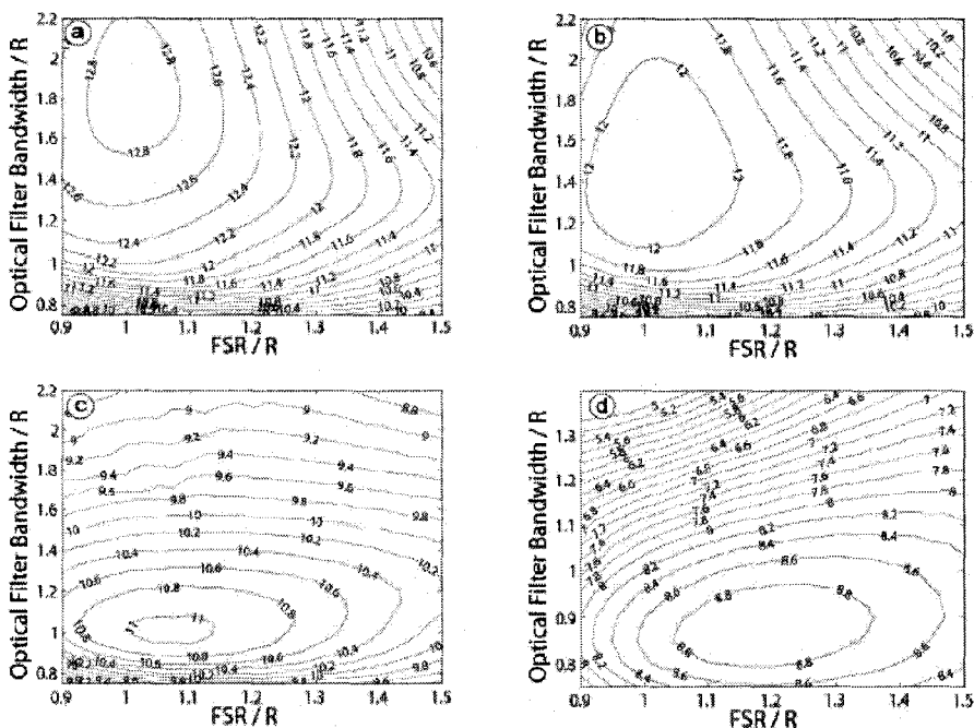
Fig. 5. CSRZ-DPSK Q-factor versus free spectral range and optical filtering bandwidth for CD index of a) 0, b) 54, c) 110 and d) 218 \times 10^3 (Gb/s) 2 ps/nm.
