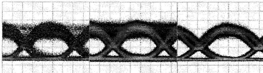
Fig. 5. Eye diagrams of the destructive port for 4 bit delay, 2bit delay and 1 bit delay demodulator. The longer delays demodulator were passive devices in our experiment making them more difficult to align the frequency of the laser to the transmission frequency of the DLI which resulted in a penalty.
