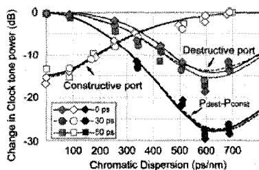
Fig. 5. OOK clock tone power change versus dispersion for different DGD values. Experiments (dots) and simulation (lines) show that DGD does not affect the change in power versus dispersion. Maximum clock tone power is at 0 ps/nm in the destructive arm and 700 ps/nm for the constructive arm. Subtracting the two curves isolates the effect of CD and increases sensitivity.
