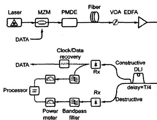
Fig. 3. Experimental setup using fiber for CD and a PMD emulator for DGD. Bandpass filters centered at 10-GHz filter out the clock tone.
