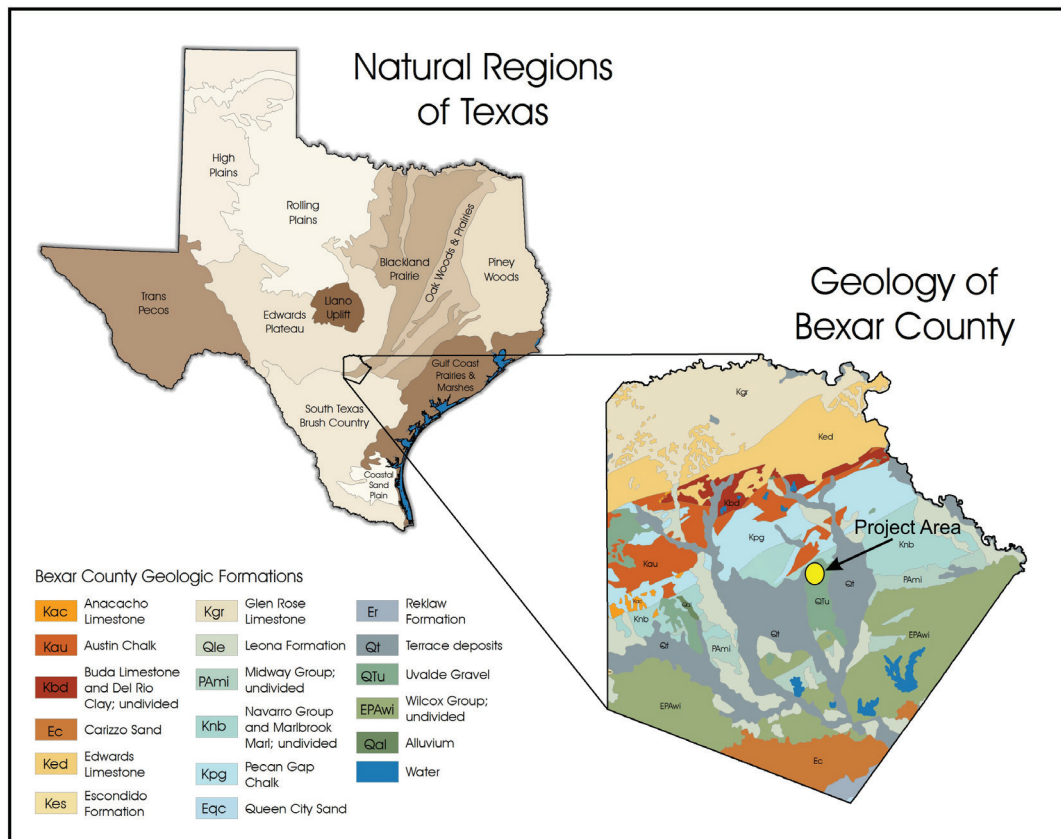
Figure 2-4. Natural Regions of Texas and Geology of Bexar County. After Mauldin et al. (2015; see also Sellards 1919).
