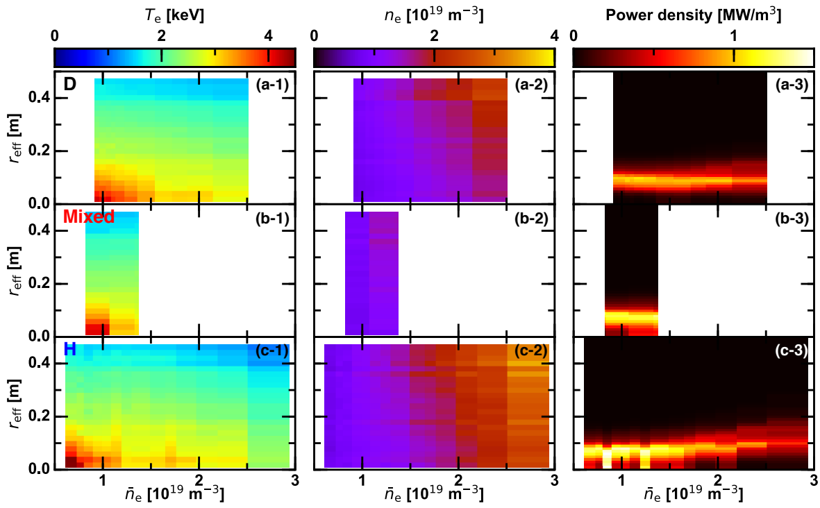
Figure 4. Line averaged density dependence of radial profiles of electron temperature (first column), electron density (second column), ECH absorption (third column) averaged in the overall analysis time period for (a) D, (b) Mixed, and (c) H plasmas.
