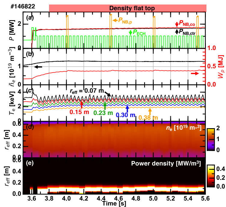
Figure 3. Time evolutions of (a) heating power, (b) line averaged density and diamagnetic plasma stored energy, (c) electron temperature, (d) electron density profile, and (e) ECH absorption profile.
