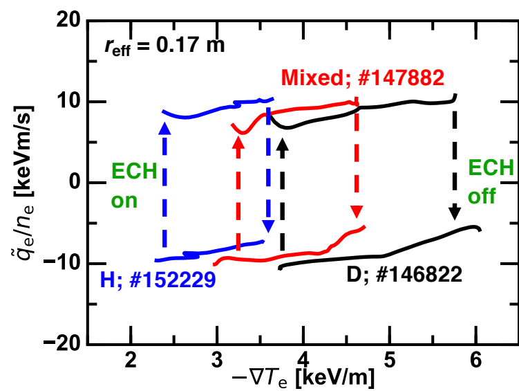
Figure 6. Trajectory of time evolution during the MECH in the flux-gradient diagram.
