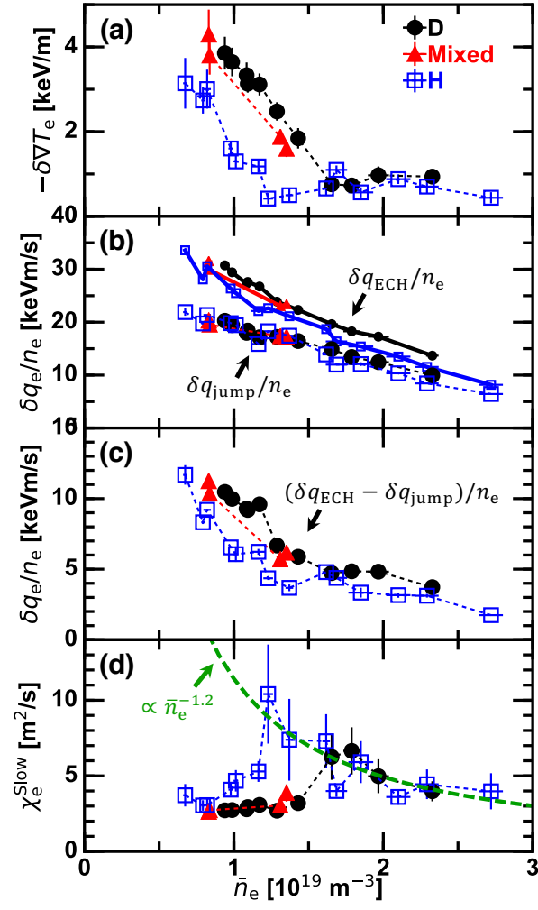
Figure 8. Line averaged density dependence of (a) the amplitude in electron temperature gradient modulation, (b) the hysteresis width \delta q_{\text{jump}} and peak-to-peak heat flux modulation amplitude \delta q_{\text{ECH}} normalized by the electron density n_e , (c) (\delta q_{\text{ECH}} - \delta q_{\text{jump}})/n_e , and (d) the slow time scale diffusivity.
