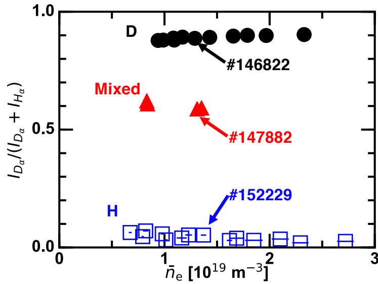
Figure 2. Experimental parameter map in the line averaged density–D/H ratio space for D, Mixed, and H plasmas. The D/H ratio is given as I_{D_\alpha}/(I_{D_\alpha} + I_{H_\alpha}) , where I_{D_\alpha} and I_{H_\alpha} are the intensity of the D_\alpha emission and the H_\alpha emission measured by a passive spectroscopy, respectively.
