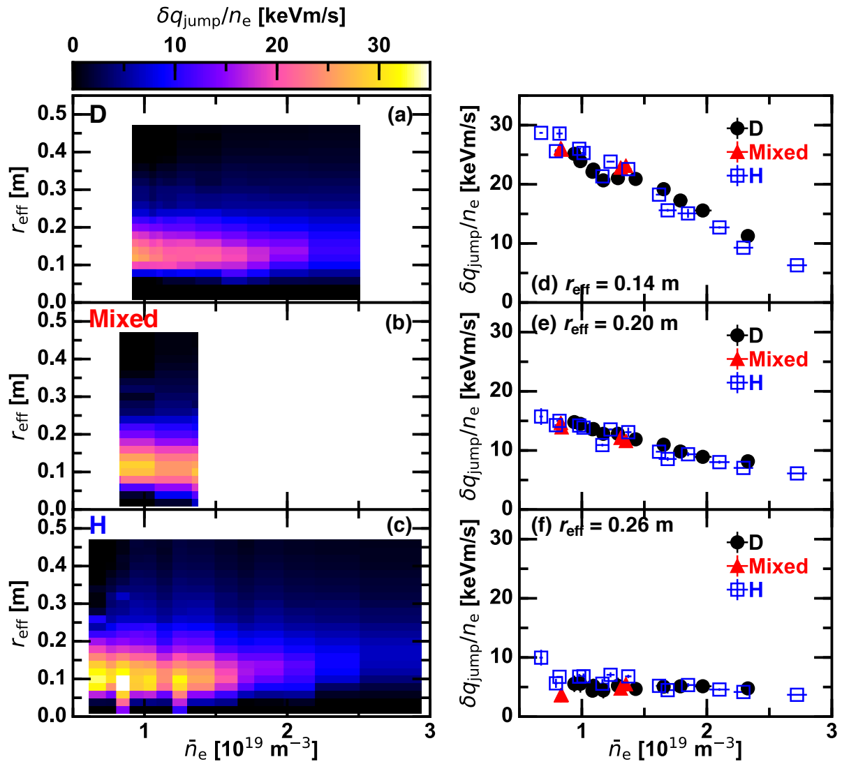
Figure 7. (Left column) Radial profile of the hysteresis width as a function of the line averaged density for (a) D, (b) Mixed, and (c) H plasmas, and (Right column) radial profile of the hysteresis width at (d) r_{\text{eff}} = 0.14 m, (e) 0.20 m, and (f) 0.26 m.
