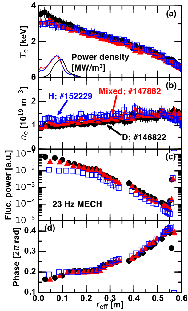
Figure 5. Radial profiles of (a) electron temperature profile and ECH power density, (b) electron density profile, and (c,d) fluctuation power being proportional to the square of the fluctuation amplitude and phase of electron temperature modulation at 23 Hz.
