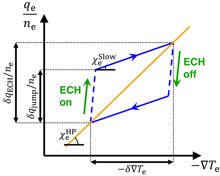
Figure 1. Schematic of the flux-gradient relation when the transport hysteresis is present.
