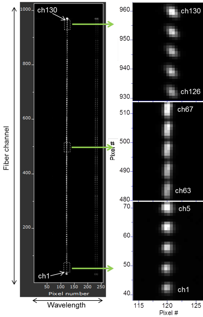
FIG.3 A CCD image of fiber array (core diameter of 50 \mu\text{m} ) taken with a 300 grooves/mm grating, an entrance slit width of 50 \mu\text{m} , an exposure time of 3 sec for 546.07 nm line of an Hg lamp. The 130 channels are aligned vertically and numbered from bottom to top. An enlarged views of the images from ch 1 to 5, ch 63 to 67 and ch126 to 130 are shown on the right panels. At the top and bottom of the image, “reference fibers” (core diameter of 115 \mu\text{m} ) are attached. These fibers are connected to a calibration lamp during the calibration of the wavelength and the LHD discharges. The images of these fibers are used to correct possible deviation of the absolute wavelength between calibration phase and the LHD experiments caused by mechanical error of the spectrometer.
