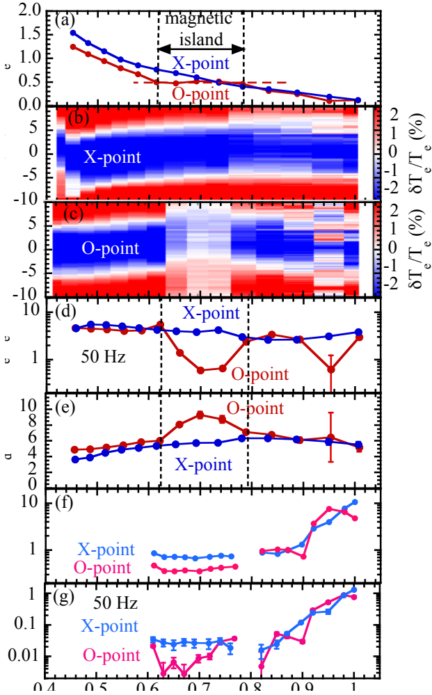
FIG. 2: Radial profiles of (a) mean T_e , the patterns of conditionally sampled signals in (b) X-point and (c) O-point phase, (d) normalized T_e modulation amplitude, \delta T_e/T_e , (e) delay time of T_e modulation ( t_d ) given by the phase shift between ECH pulse and T_e modulation, (f) \tilde{n}/n levels measured with BES, and (g) \tilde{n}/n modulation amplitude, \delta(\tilde{n}/n) levels, in the O-point phase and X-point phase.
