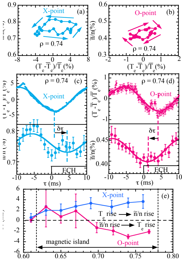
FIG. 3: Hysteresis of amplitude between \tilde{n}/n and T_e modulation at \rho = 0.74 in the (a) X-point and (b) O-point, time evolution of T_e and \tilde{n}/n at \rho = 0.74 in the (c) X-point and (d) O-point phase with the relative time ( \tau ) respect to the onset of ECH, and (e) radial profiles of delay time difference between modulation of T_e and \tilde{n}/n ( \delta\tau ) at X-point phase and the O-point phase.
