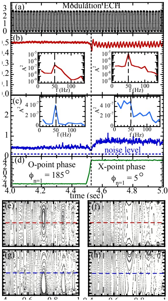
FIG. 1: Time evolution of (a) power of ECH, P_{ECH} (b) T_e measured with the ECE at \rho = 0.74 , (c) \tilde{n}/n integrated from 10 kHz to 50 kHz at \rho = 0.74 , and (d) current of C-coil and Poincaré map at the poloidal cross section of T_e measurements in (e) O-point and (f) X-point phase and Poincaré map at the poloidal cross section of \tilde{n}/n measurements in (g) O-point and (h) X-point phase. The frequency spectrum of T_e modulation and envelope of density fluctuation are also plotted in Figure (b) and (c).
