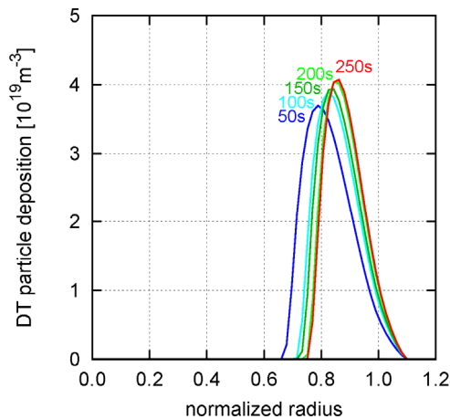
Figure 13. Time evolution of the radial profile of the pellet ablation for sub-ignition operation. After reaching the steady-state ( t > 250 s), the deposition profile also becomes constant.
