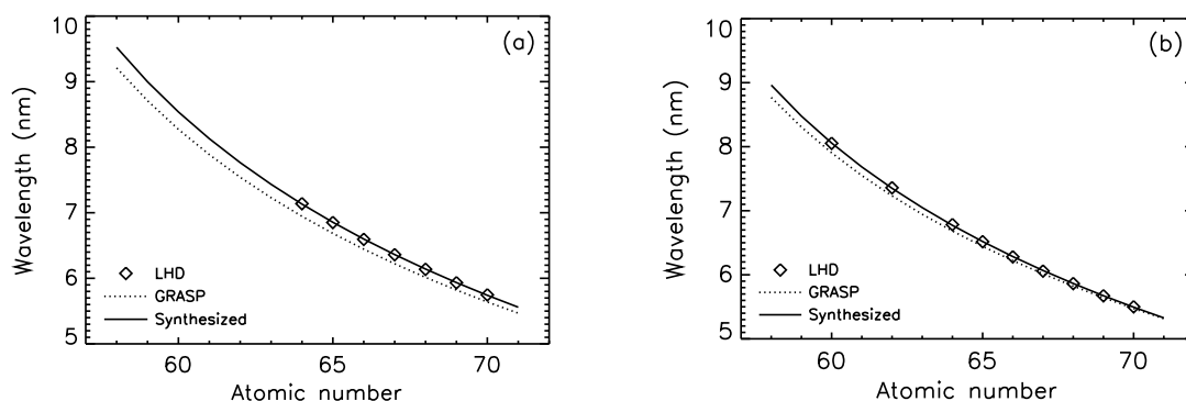
Figure 2. Atomic number dependences of the wavelengths for the transitions (a) 4d^{10}4f^2F_{7/2}-4d^94f^2^2G_{9/2} of Ag-like ions and (b) 4d^{10}1S_0-4d^94f^1P_1 of Pd-like ions. The wavelengths measured in the LHD are plotted with diamond symbols, while those calculated by GRASP92/RATIP are drawn with dotted lines. Solid lines denote the wavelengths synthesized with the fitting (see the text in Section 5 for details).
