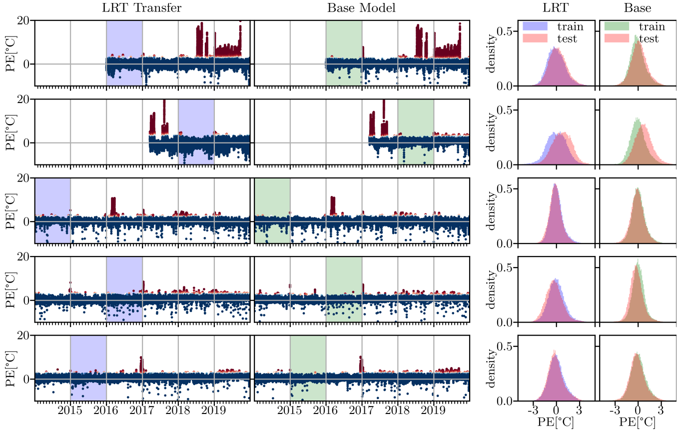
Figure 4. Scaling up FD training using TL within the farm. Each row displays the results of TL to another target turbine, all with the same source turbine. Two left columns: PEs for the LRT transfer framework, PEs using the base CNN model to train from scratch on the target turbine data. Two right columns: the corresponding PE distribution comparison between train and (healthy) test set for each training scheme. Color code: green for training from scratch, blue for TL, red for testing. The training or tuning periods are marked with the corresponding color in the left two columns.
