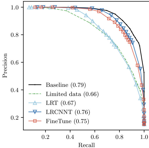
Figure 6. Precision-Recall curves for cross-farm TL. The source and the target turbines are from two different wind farms. The FD performance scores of the TL frameworks are compared with the baseline training scheme (solid black), and with the limited data scheme (dashed green), where the base CNN model is trained with 1 year and with 3 months of data from the target turbine respectively. Average precision values (area under curve) are stated in brackets for each training scheme.
