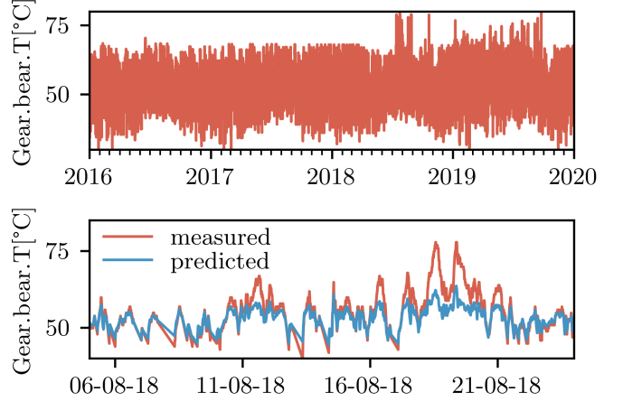
Figure 1. Raw gearbox bearing temperature of the turbine T_0 . Lower panel: zoom in of the measured and predicted values when training the base CNN model with one year of data from this turbine (baseline training scheme).
