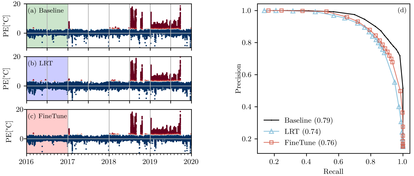
Figure 3. Comparison of approaches for TL between turbines within one farm. Prediction errors (PEs) are plotted vs. time for three training schemes: (a) baseline training of the base CNN model from scratch on target turbine data (b) LRT framework for TL (c) FineTune framework for TL. Both TL frameworks are between turbines from the same wind farm. PEs are colored red when the fault detection threshold using significance level \alpha = 0.01 is exceeded. The training or tuning period (1 year) is marked with colorful background. panel (d): Precision-Recall curves for the 3 training schemes of panels (a)-(c). Average precision values (area under curve) are stated on the legend in brackets.
