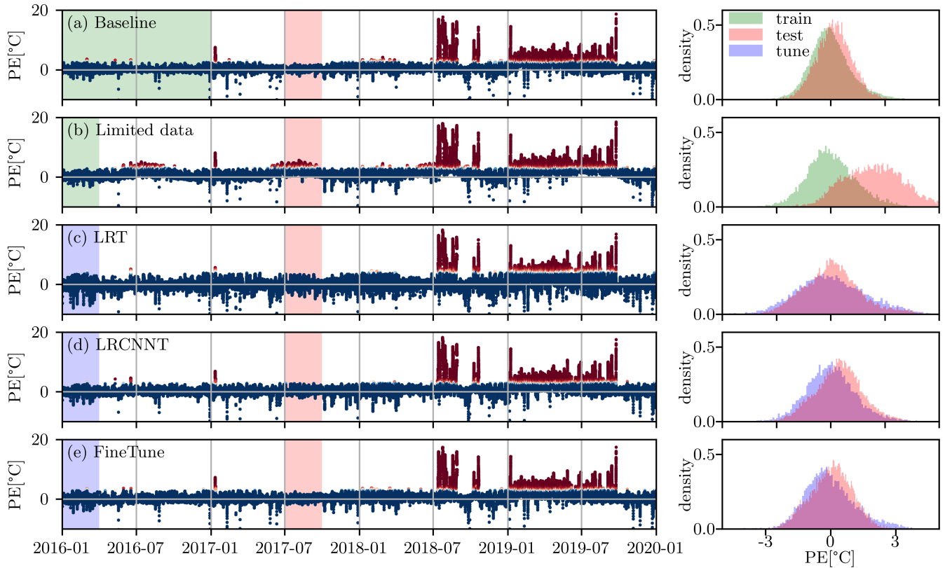
Figure 5. Comparison of different training schemes for cross-farm TL. Time dependent PEs (left column) and their distributions (right column) for 5 training schemes for FD on the same target turbine T_0 . The baseline (a) and Limited data (b) schemes correspond to training from scratch of the base CNN model with 1 year and 3 months data respectively. In the TL frameworks LRT (c), LRCNNT (d) and FineTune (e) the base model is pre-trained with data from a source turbine S_1 of another wind farm and then tuned using the different TL frameworks to obtain PEs for the target turbine. Color code: green for training from scratch, blue for TL, red for testing. The training, tuning and testing periods are marked with the corresponding background color in the left column.
