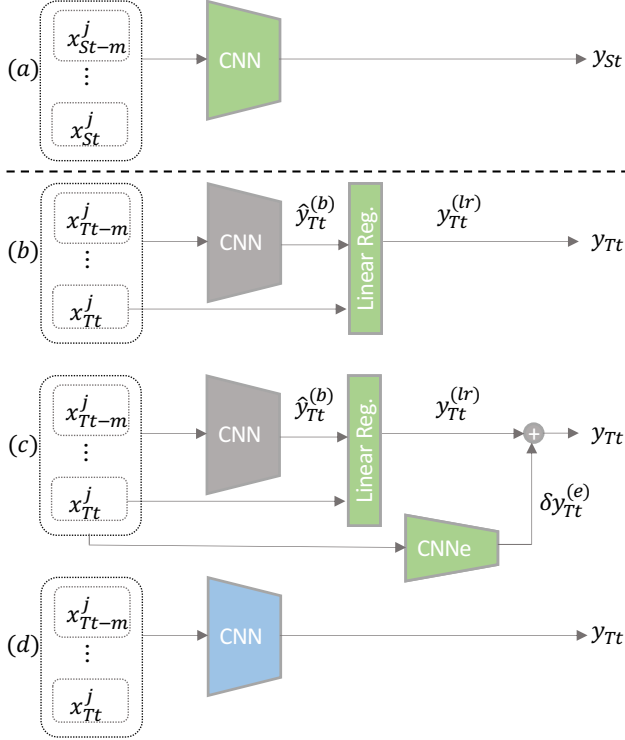
Figure 2. Training schemes for TL of CNN- based fault detection. (a) Pre-training of the base model with data from the source turbine. (b)-(d) the 3 TL schemes suggested in the paper for tuning the model to predict on target turbine data: (b) LRT (c) LRCNNT (d) Fine Tuning. Training from scratch, fine-tuning of pre-trained weights and no training (fixed weights) are colored green, blue and gray respectively.
