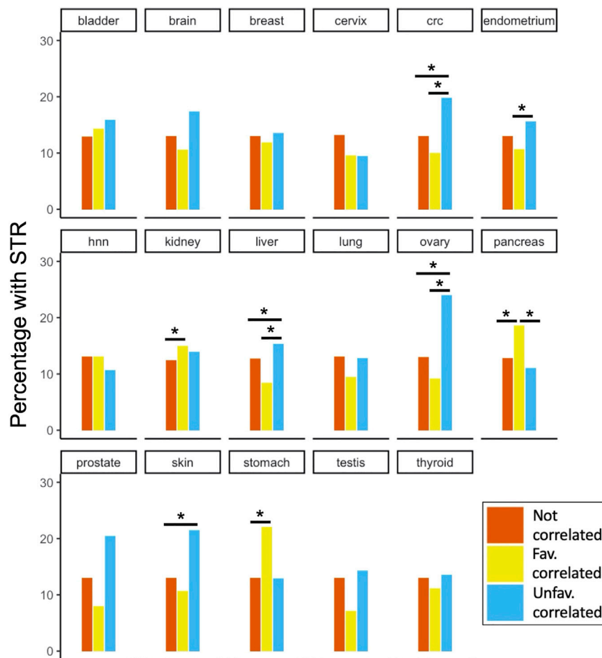
FIGURE 5 | STR-containing proteins and their correlation to patient survival in cancer. For all 17 cancer types included in the Protein Atlas Pathology Atlas, the percentage of STR-containing proteins among the proteins that were either uncorrelated or correlated (un-)favourably with patient survival are shown. Significant enrichments after Benjamini-Hochberg FDR correction are marked with asterisks. Note that while percentages are shown in the plot for clarity, tests were performed on absolute numbers of proteins. Abbreviations: hnn, head and neck; crc, colorectal cancer.
