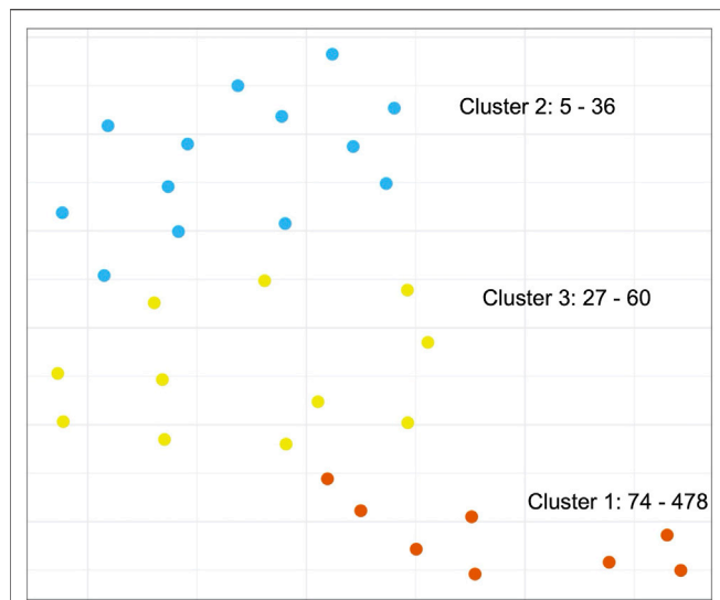
FIGURE 6 | Clustering of biological functions of STR-containing proteins in the Protein Atlas Pathology Atlas. K-means clustering of the UMAP-embedded number of STR-containing proteins associated to Gene Ontology terms for all PA groups. Text annotations in the graph refer to the PA groups in each cluster with the smallest and largest number of STR-containing proteins. Note: while clustering was performed on a 10-dimensional embedding, the results are visualized here using a 2-dimensional embedding.
