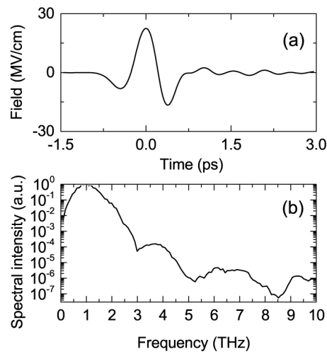
Fig. 2. Broadband terahertz radiation. (a) Optical rectification of the transform-limited pump pulse in the organic crystal OH1 gives rise to a single-cycle terahertz field carrying a broad spectrum between 0.1 and 3 THz. (b) The field shape and spectral intensity are reconstructed in free-space electro-optical sampling carried out in a 200- \mu\text{m} thick GaP crystal.
