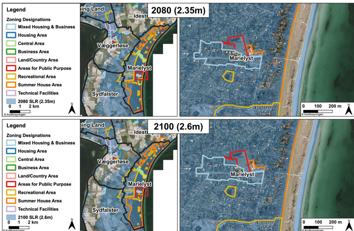
Figure 10. Projections for the Marielyst area for 2080 and 2100 scenarios.
