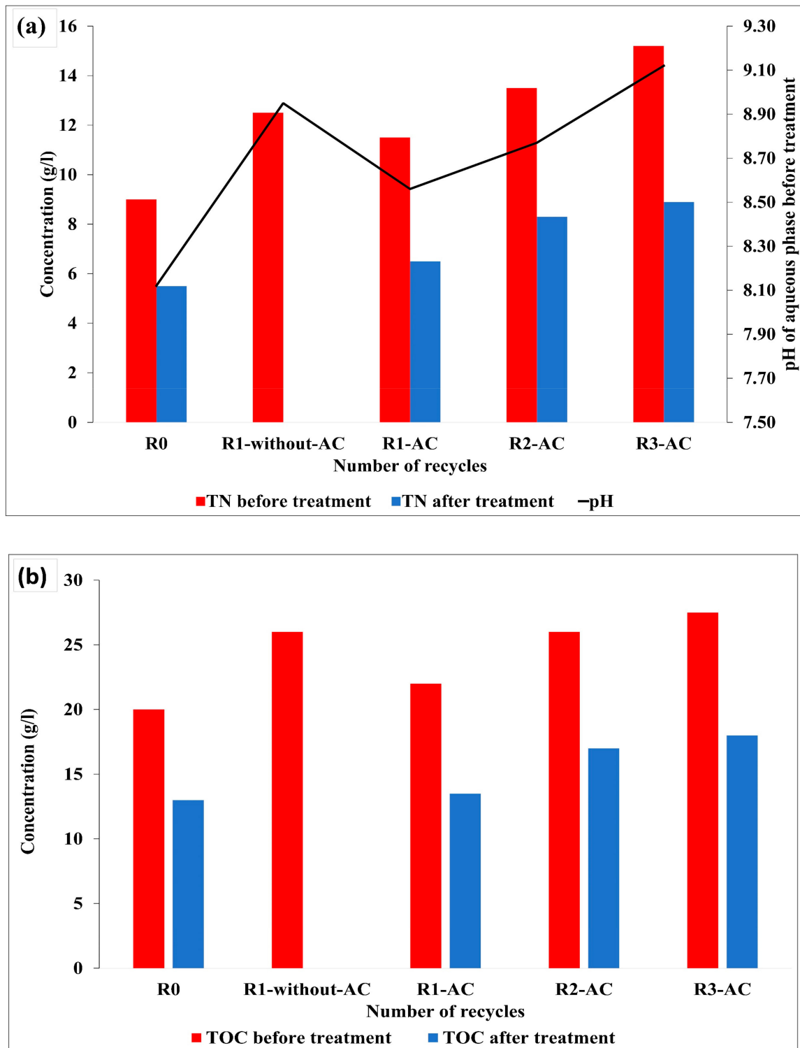
Figure 3. Effect of AC treatment on the concentration of (a) TN and (b) TOC.
