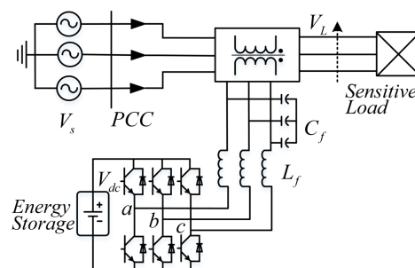
Fig. 1: Circuit diagram of a DVR configuration
