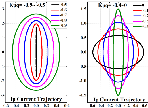
Fig. 7: I_p current trajectories with k_{pq} where -1 < k_p = -k_q = k_{pq} < 0 in \alpha\beta system
