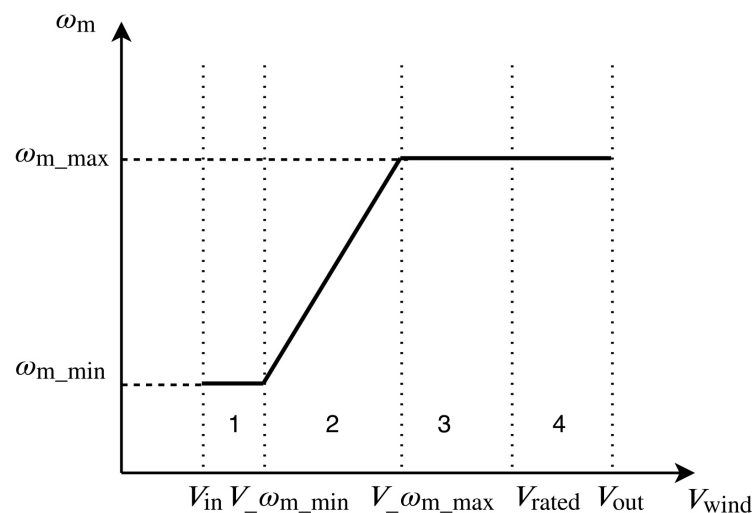
Figure 6. Speed curve based on four speed regions.
