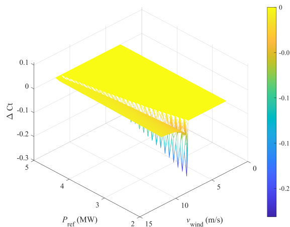
Figure 10. \Delta C_t between different derating strategies.
