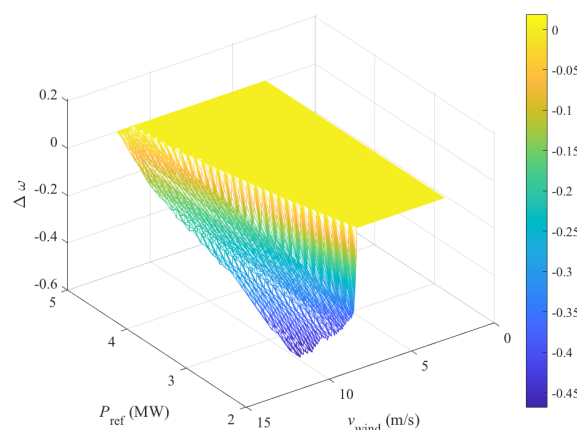
Figure 9. \Delta\omega between different derating strategies.
