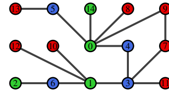
Fig. 2: Graph partitioned into 3 sets.
