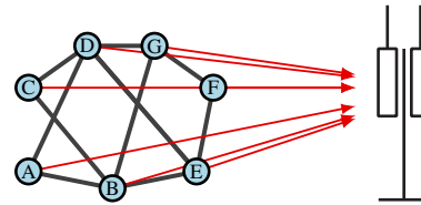
Fig. 1: Concept drawing of the system on a slice of the test network. Communication between base station and sensors (red arrows) and associations between sensors (black lines).
